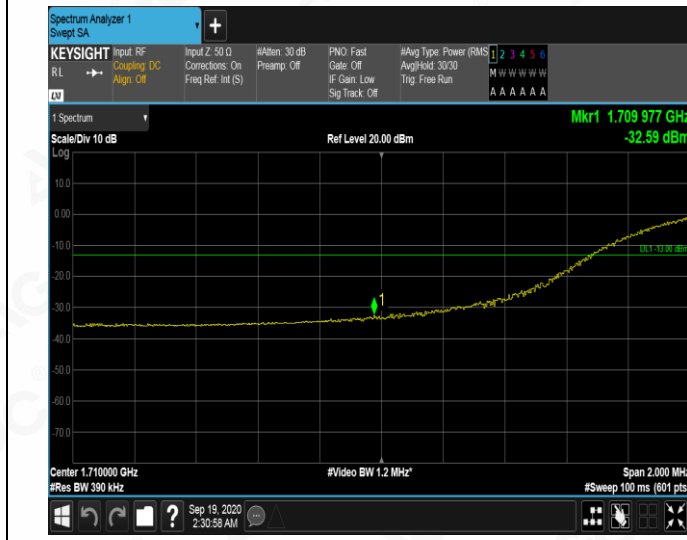
LCH_QPSK_100RB#0
