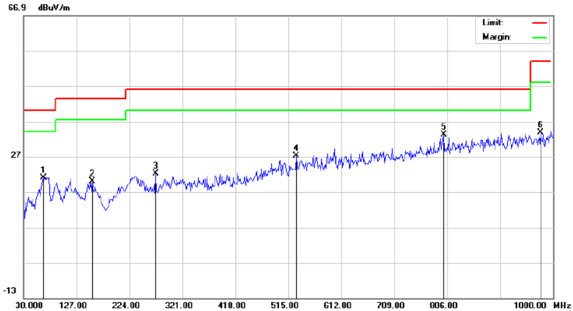
Radiated Emission Test –Horizontal -3m Below 1G
