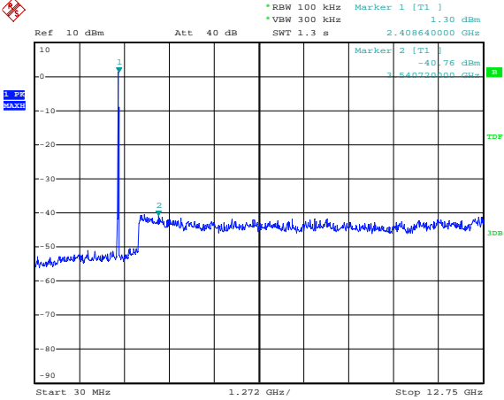
Figure 6. Plot of the Spurious RF conducted emissions 802.11b
