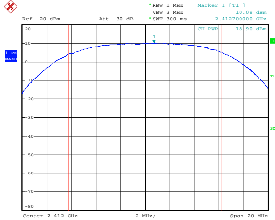
Figure 1. Plot of the Maximum Peak Output Power 802.11 b
