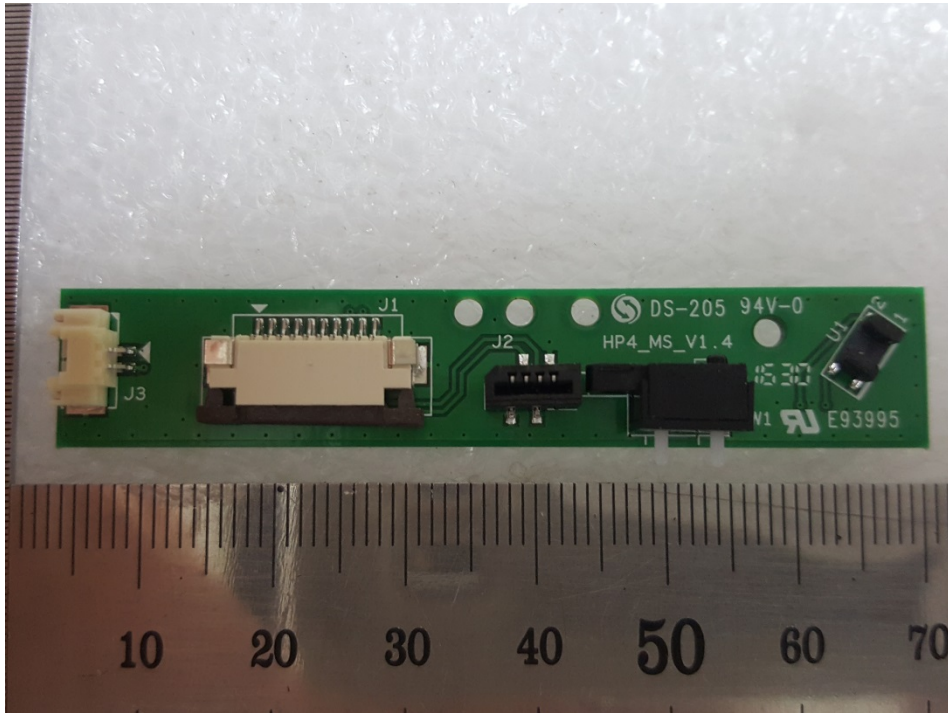
View of Main Sub Board (TOP)
