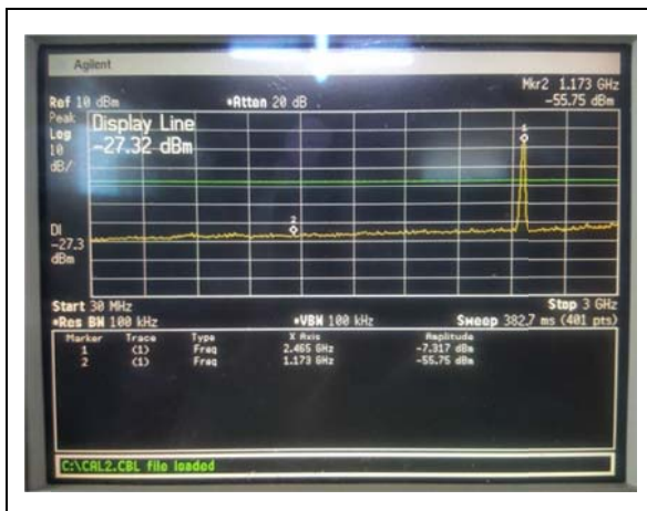
Highest Channel: 30 MHz ~ 3 GHz
