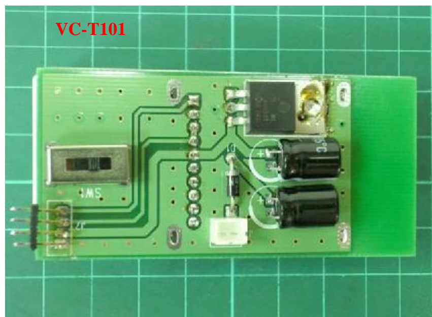
Photo 2: Inner view
