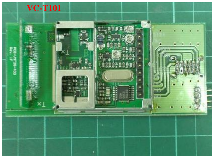
Photo 3: Inner view
