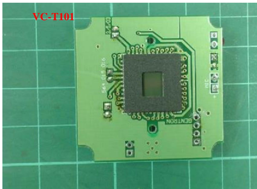
Photo 5: Inner view
