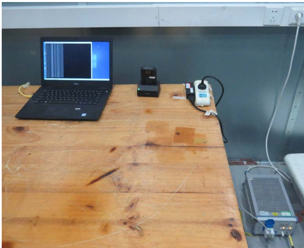
Picture 2 Conducted Emission Test Setup
