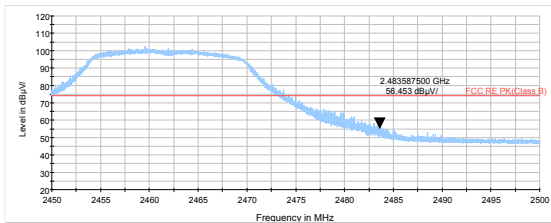
802.11g-Channel 11 Peak
