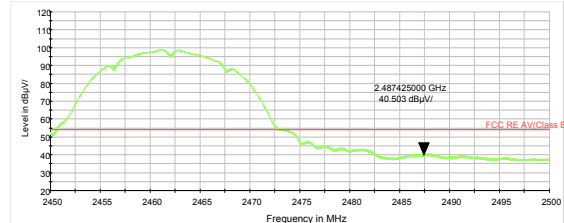
802.11b-Channel 11 Average
