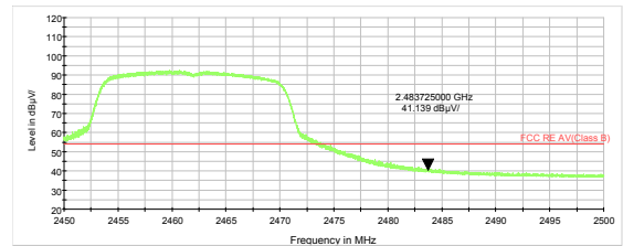
802.11g-Channel 11 Average
