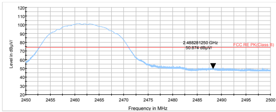
802.11b-Channel 11 Peak
