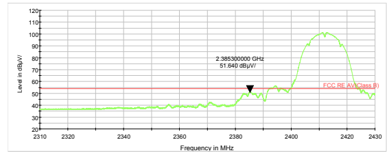
802.11b-Channel 1 Average
