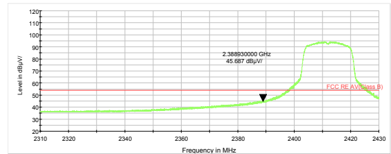
802.11g-Channel 1 Average
