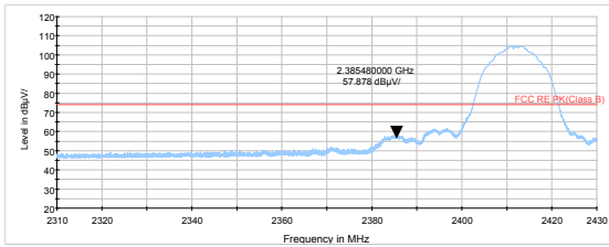
802.11b-Channel 1 Peak
