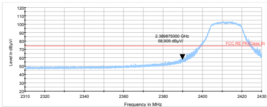
802.11g-Channel 1 Peak
