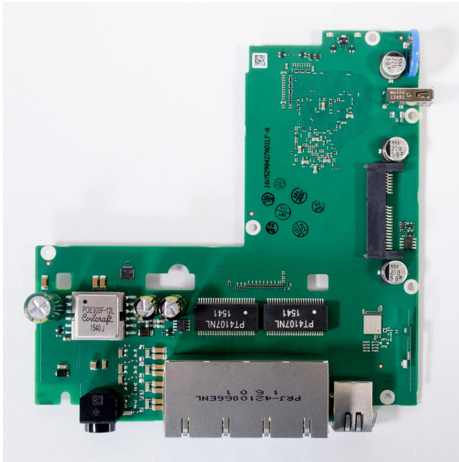
Top side of the PCB
