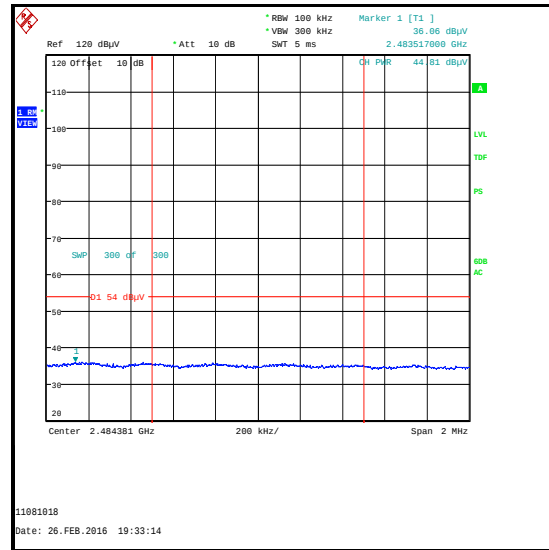
Unwanted Emission at 2484.381 MHz Average Measurement / Integration Method
