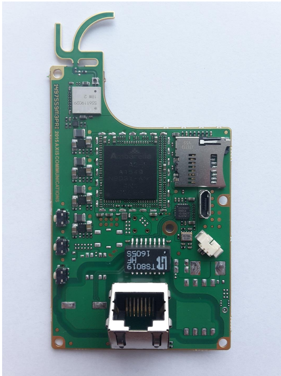
Bottom side of PCB without shield can
