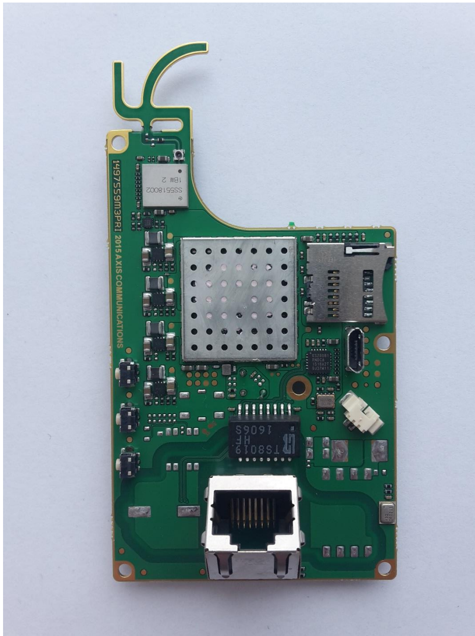
Bottom side of PCB
