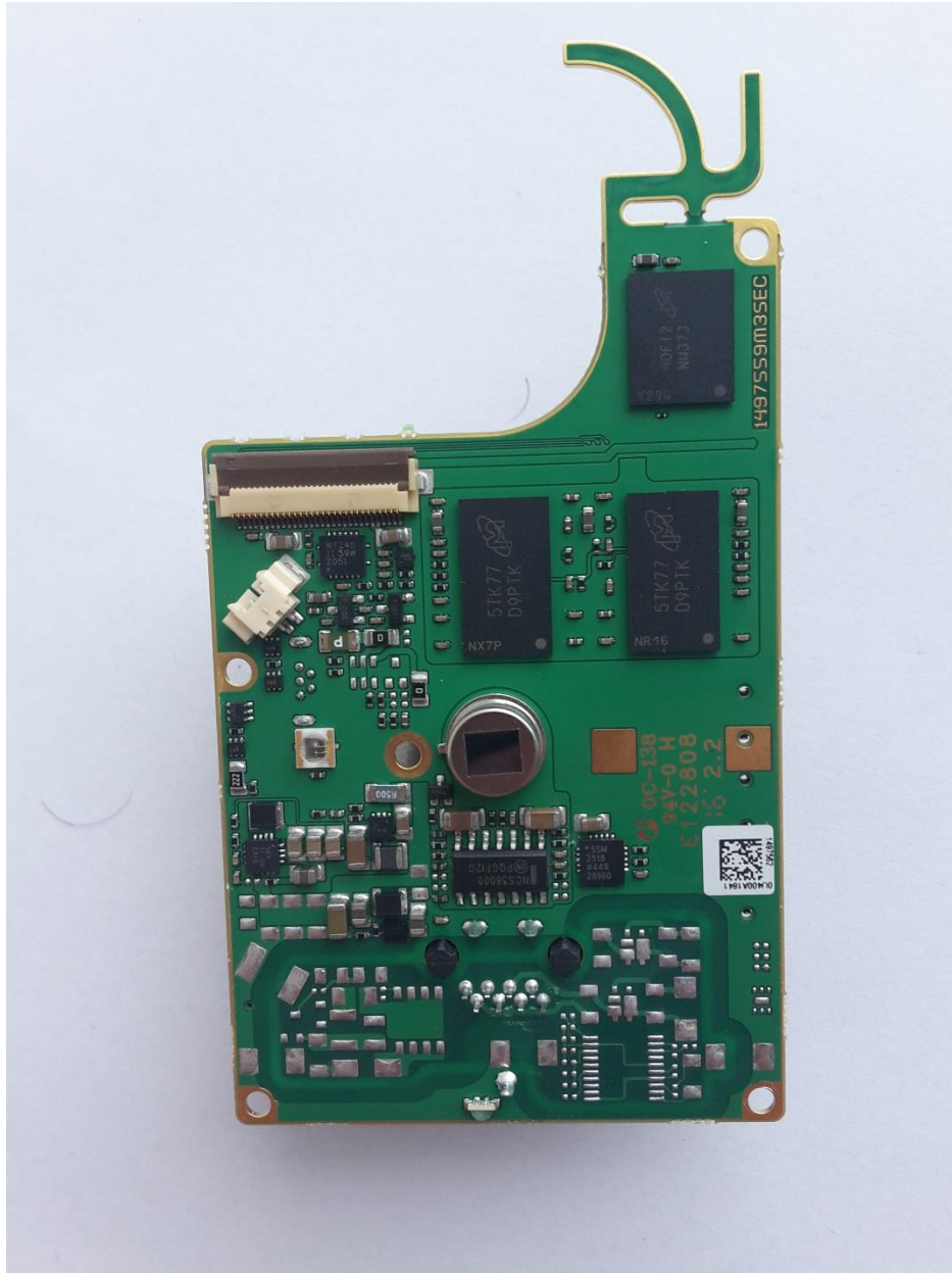
Top side of PCB
