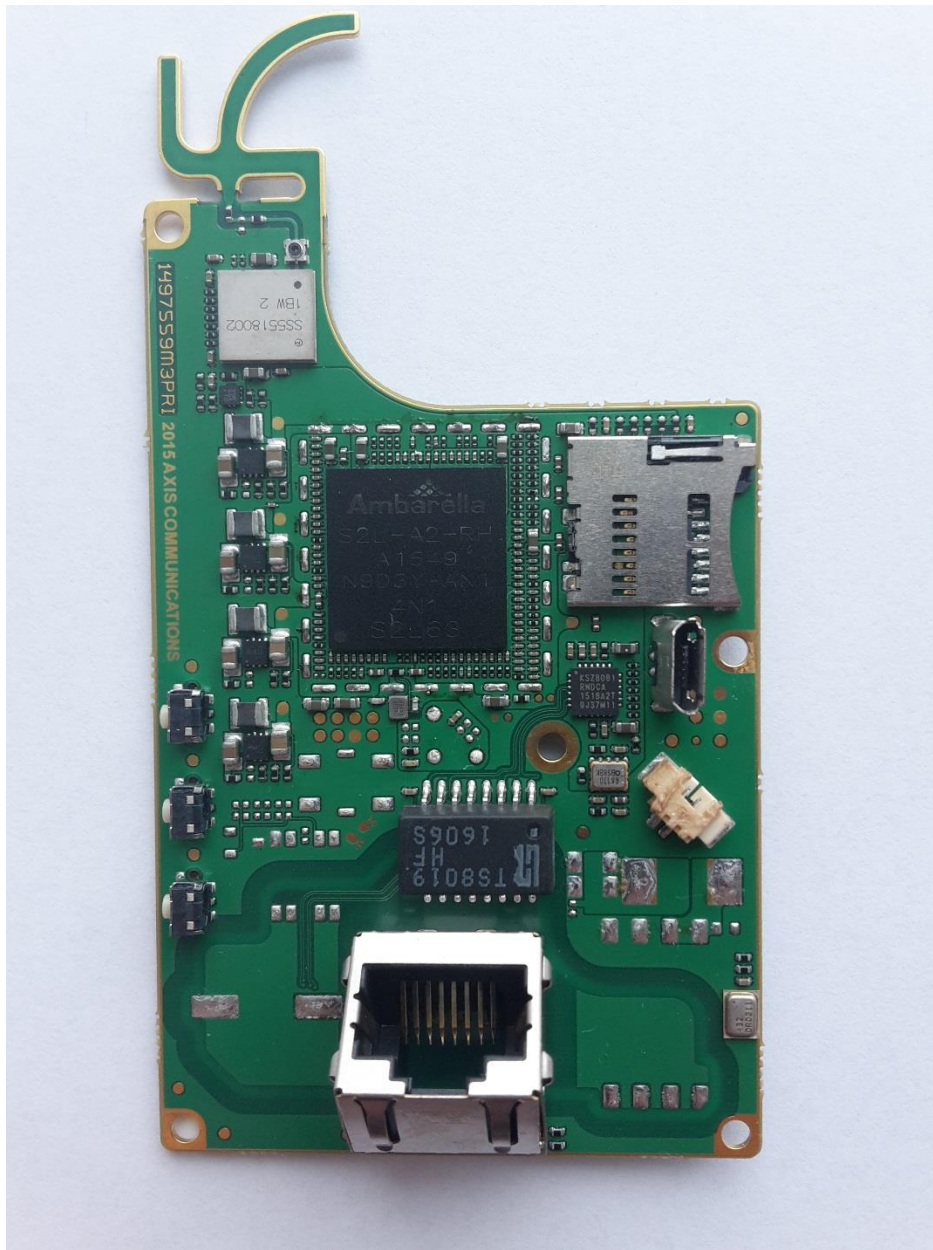
Bottom side of PCB without shield can
