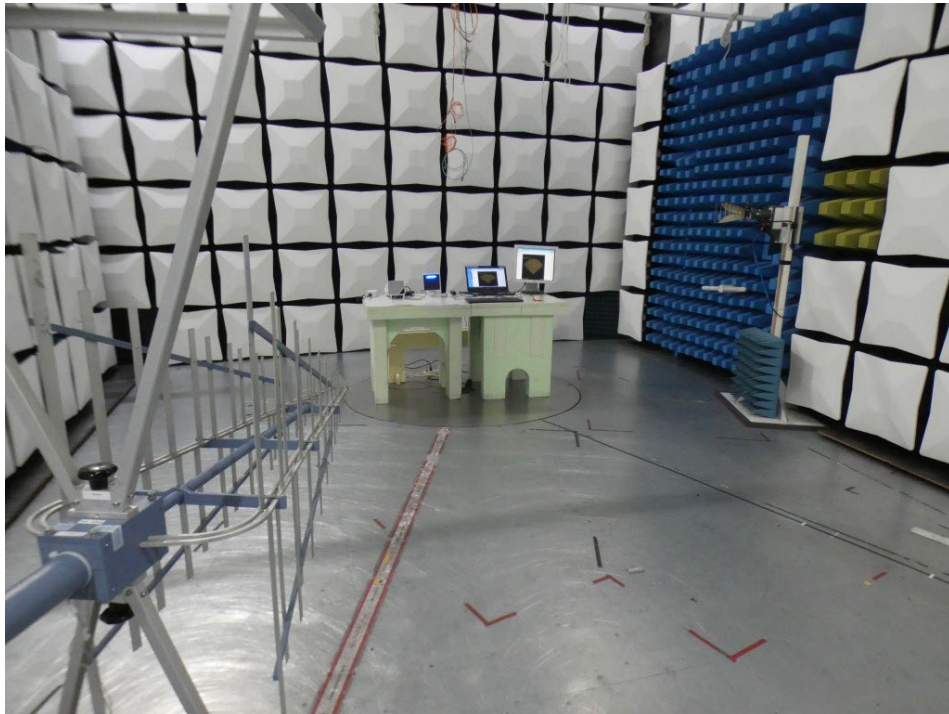
Photo 1: Test setup with S01_AB01 (computer peripheral setup) for radiated emissions measurements below 1 GHz in the semi anechoic room (SAR)
