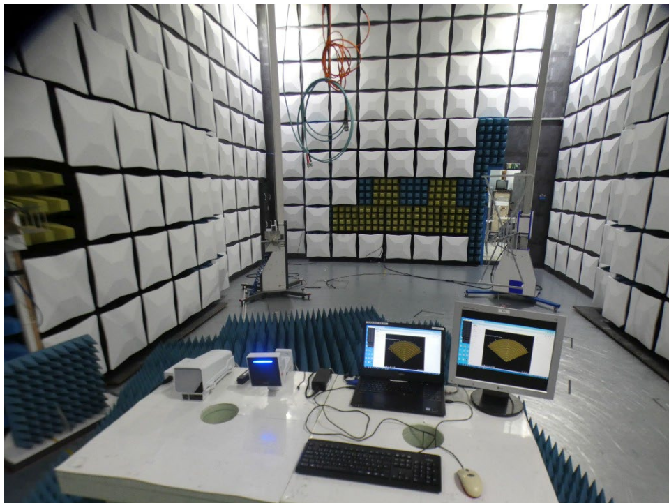
Photo 2: Test setup with S01_AB01 (computer peripheral setup) for radiated emissions measurements - above 1 GHz in the semi anechoic room (SAR)
