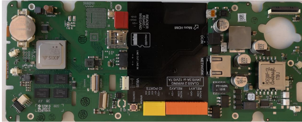
Primary side of the Main board
