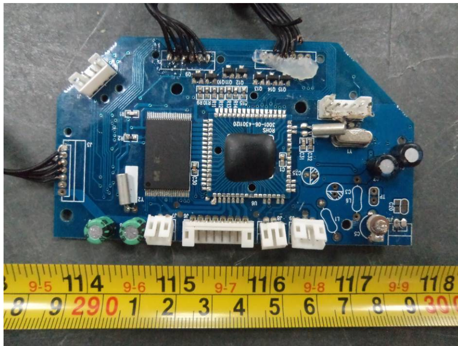
EUT -3001-06-1501120 Board Top View
