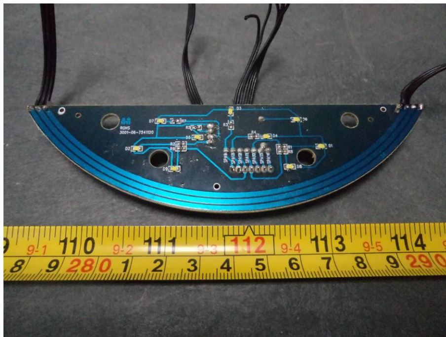
EUT -3001-06-7541120 Board Top View
