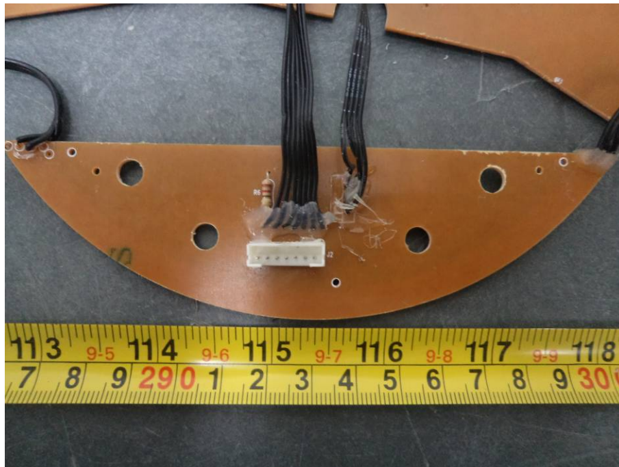
EUT -3001-06-7541120 Board Bottom View
