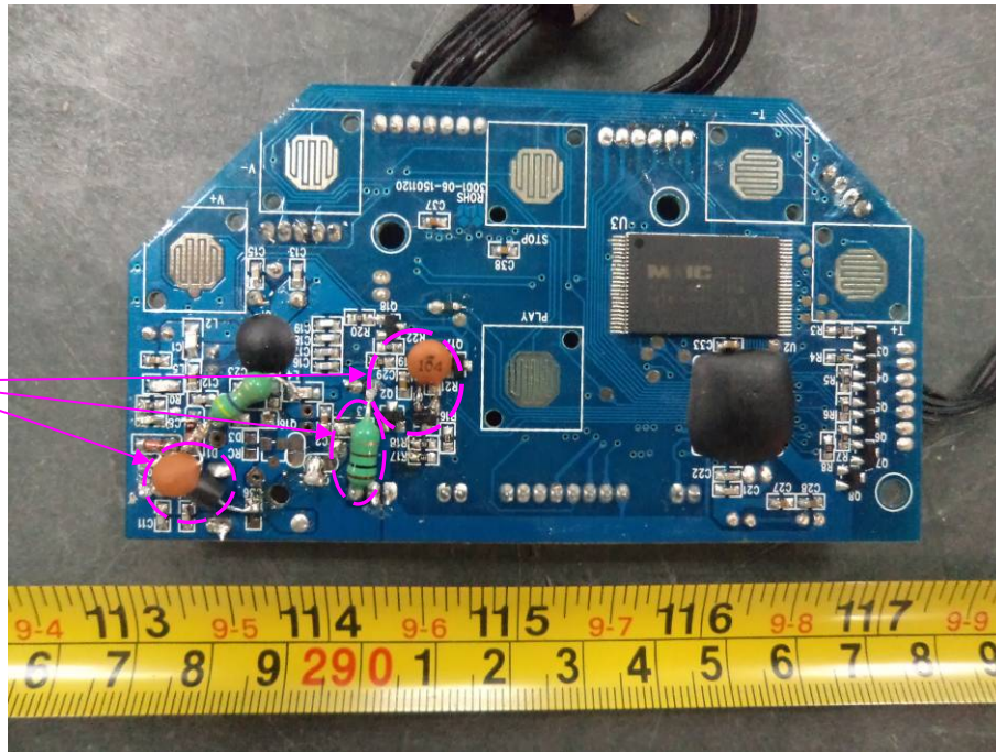
EUT -3001-06-1501120 Board Bottom View
