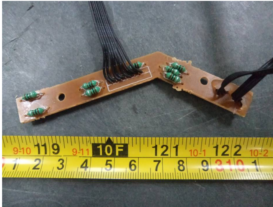
EUT -3001-06-751120 Board Bottom View
