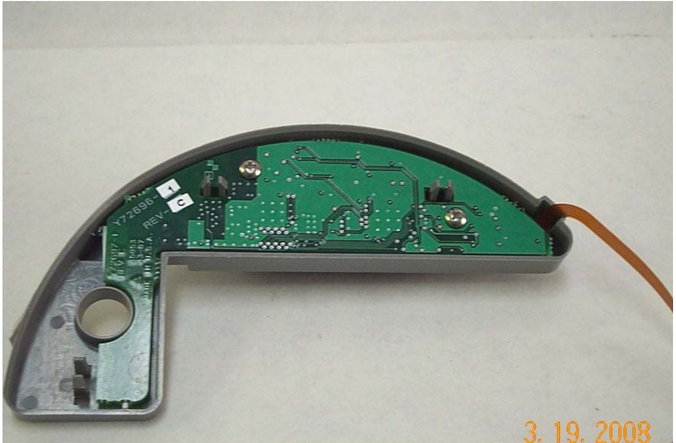
EUT installed in cover.
