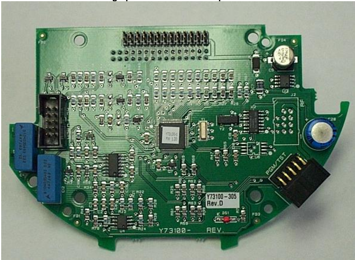
Photograph of Y73100-305 Foil Side
