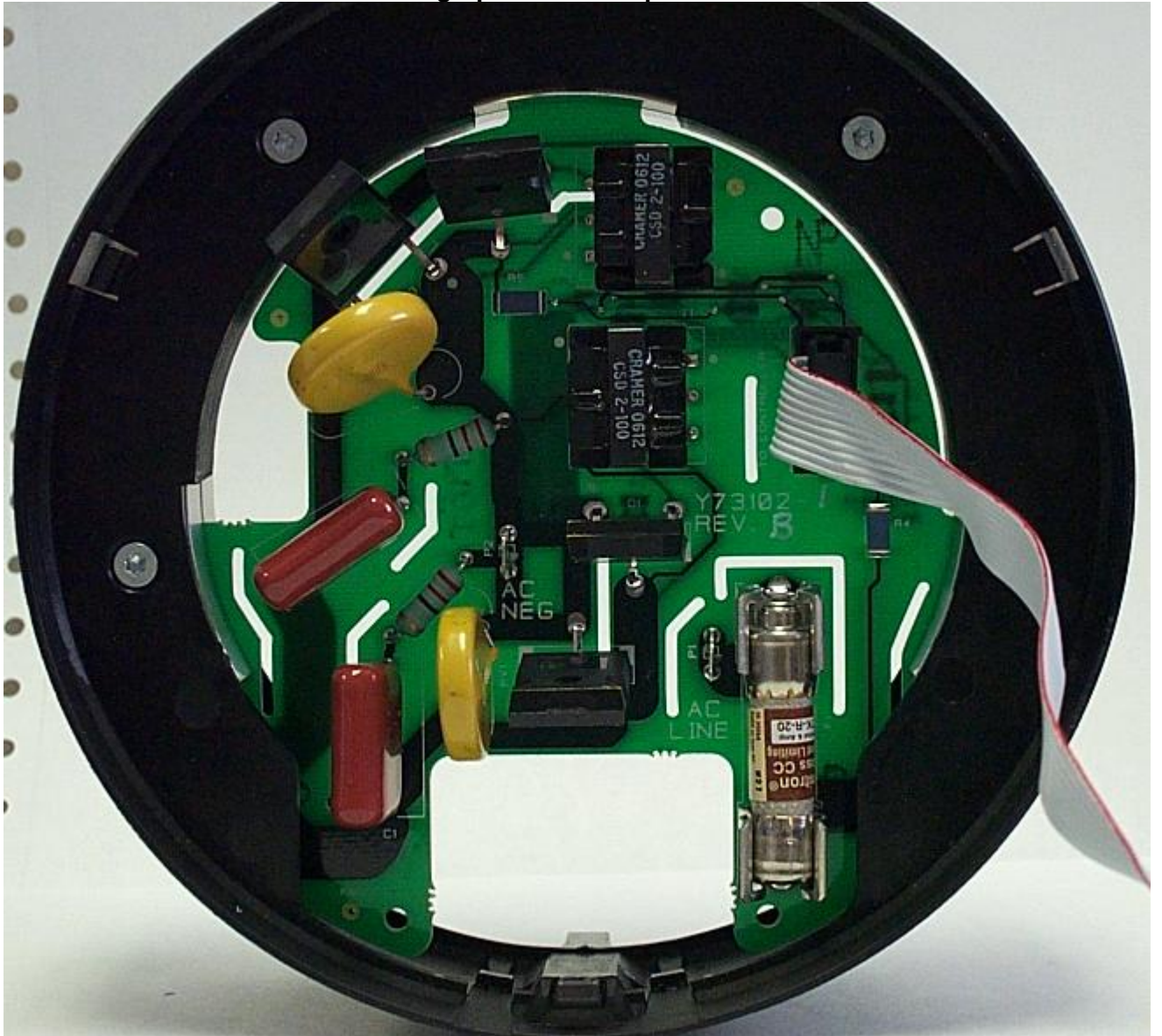
Photograph of XX Component Side
