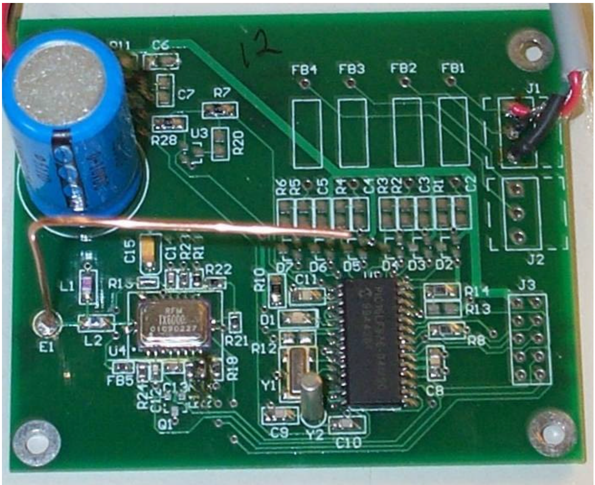
Component Side of PC Board
