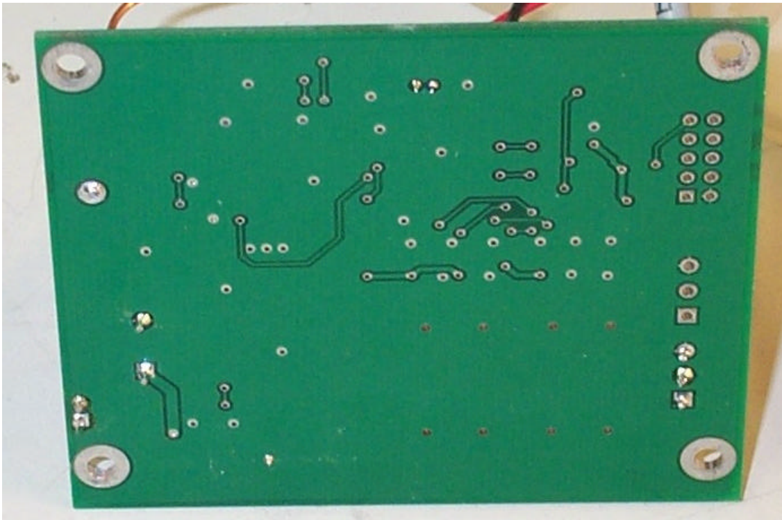
Foil side of PC Board
