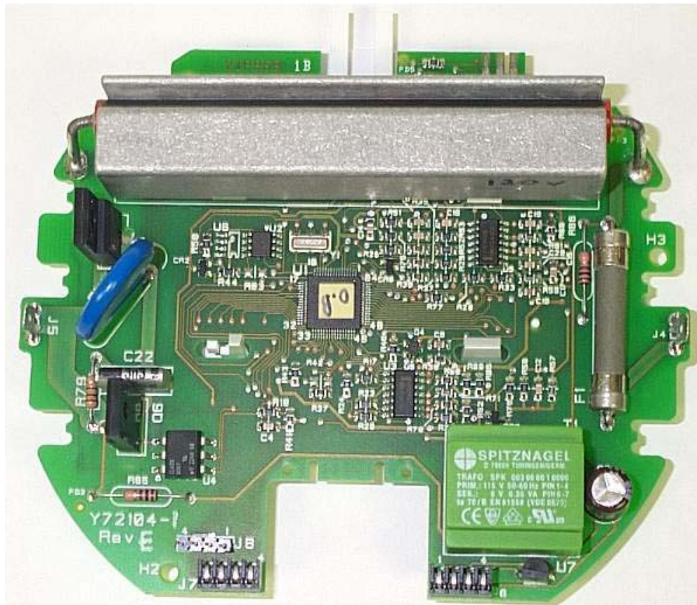
Electricity Meter PCB Side 1
