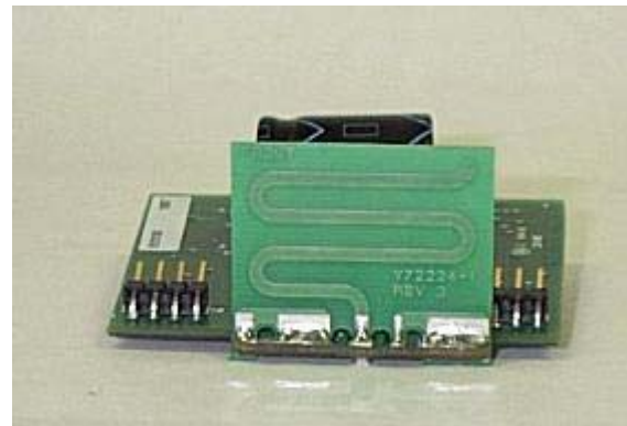
Antenna: Front Side
