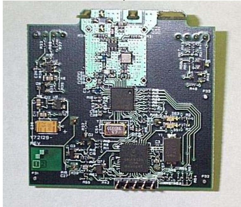
EMTR Component Side
