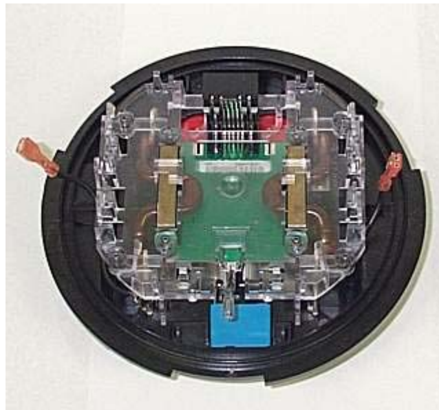
Base of Electricity Meter
