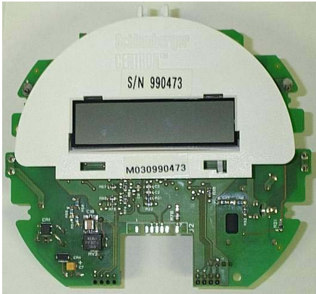
Electricity Meter PCB and Display
