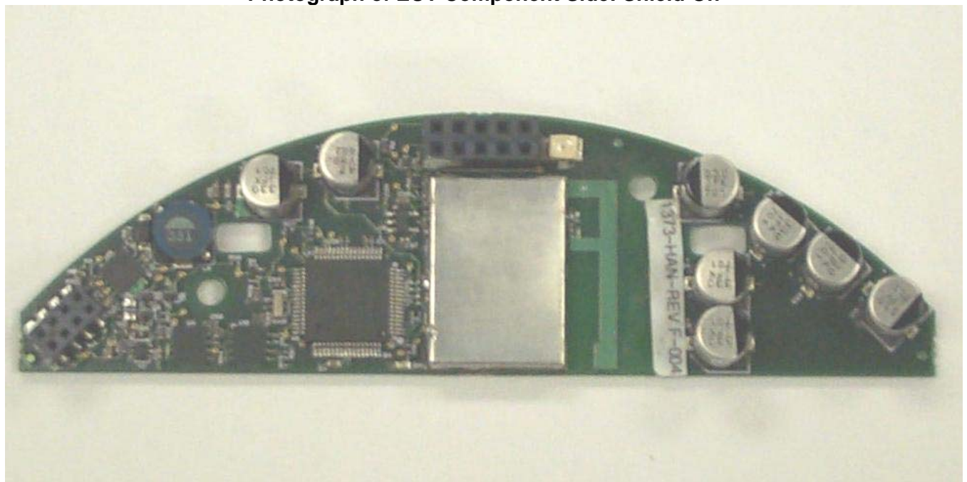
Photograph of EUT Component Side: Shield On
