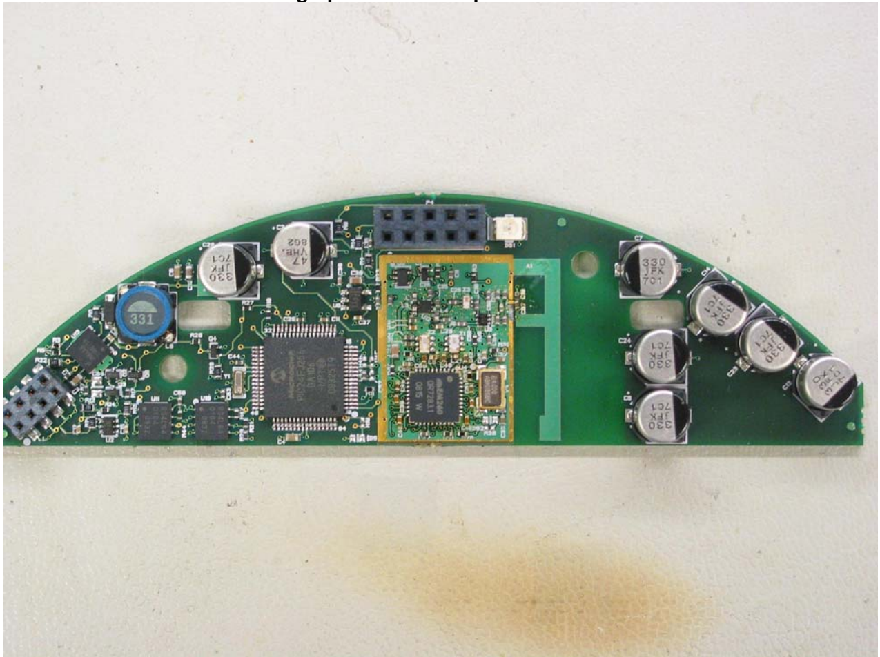
Photograph of EUT Component Side: Shield Off
