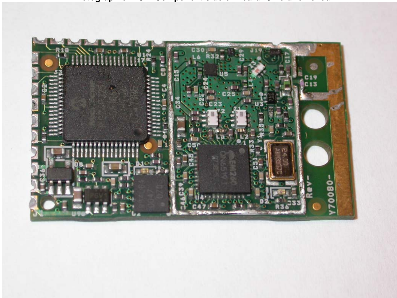
Photograph of EUT: Component side of Board: Shield removed
