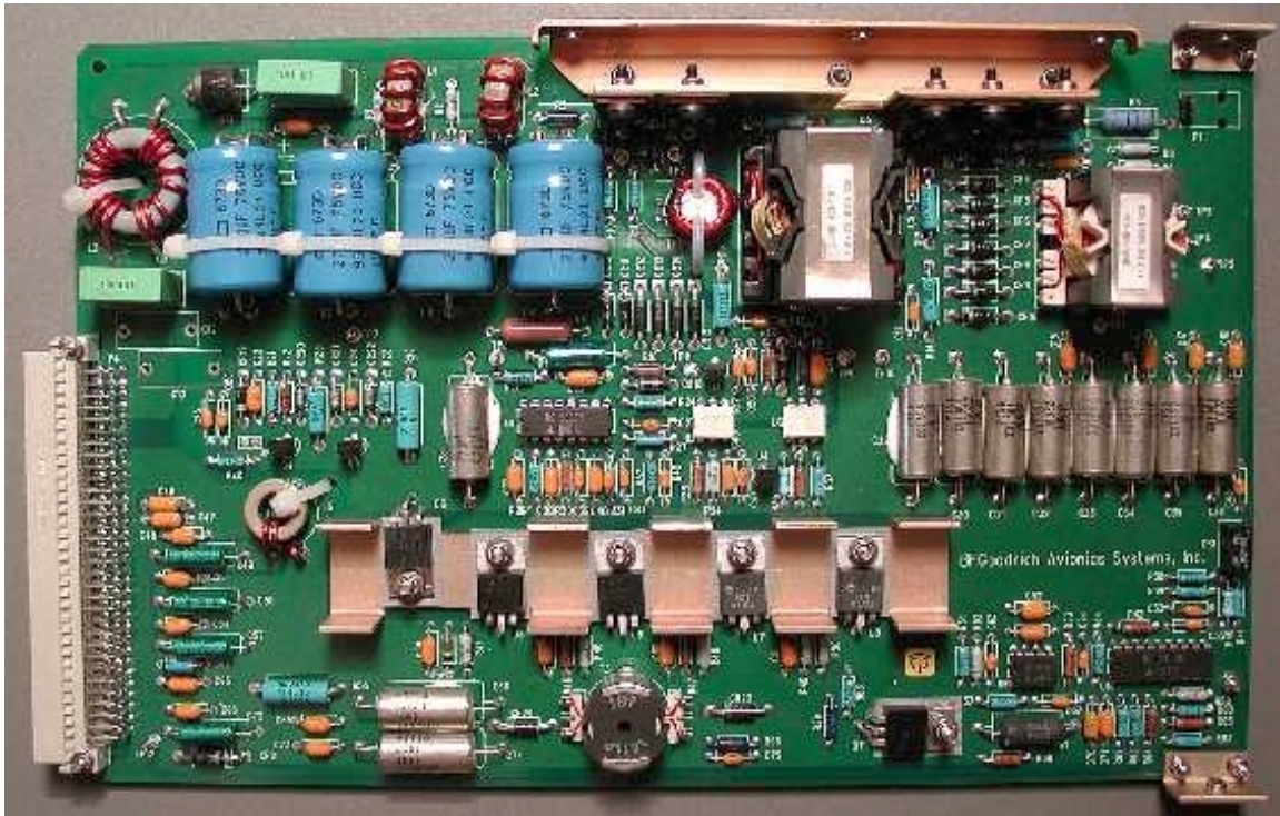
This is the top side of the power supply board.
