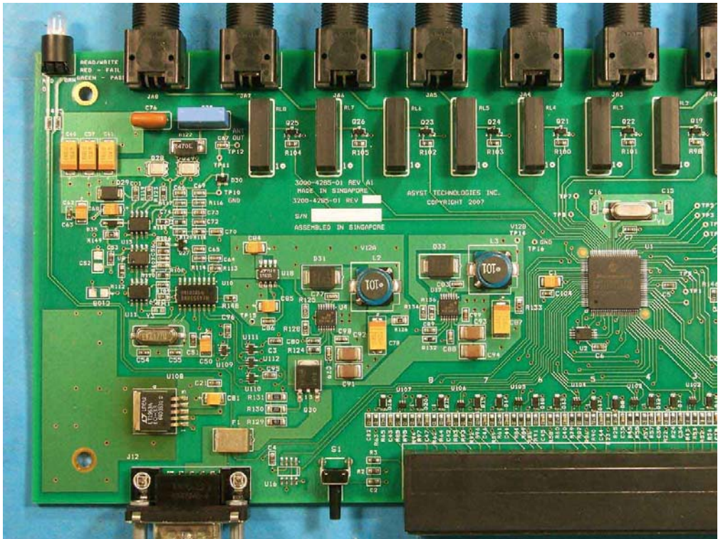
PCB Top, left half
