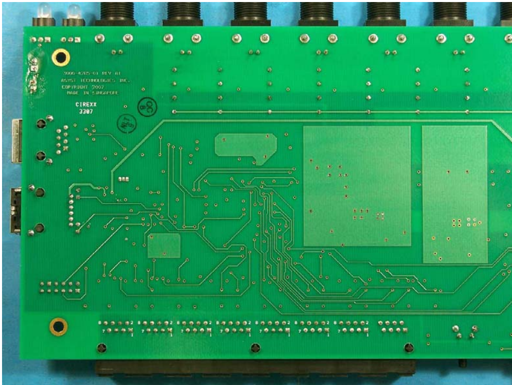
PCB Bottom, right half
