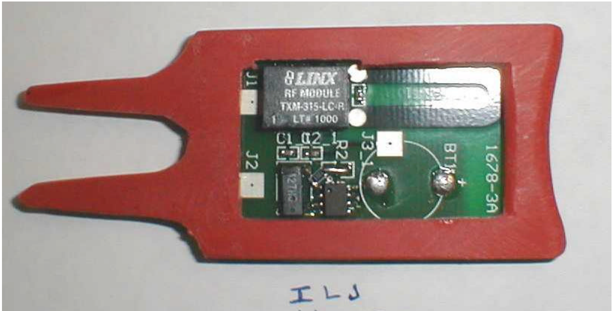
PCB Back
