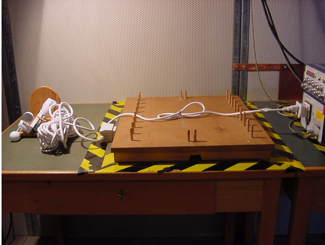
Photo 4 (Conducted Emissions):
