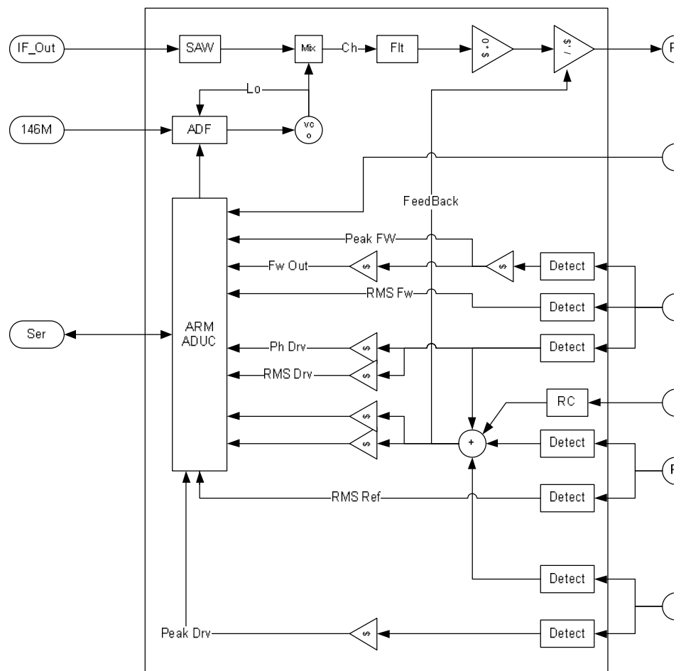
Figure 3 Echo 2 up-converter block diagram
