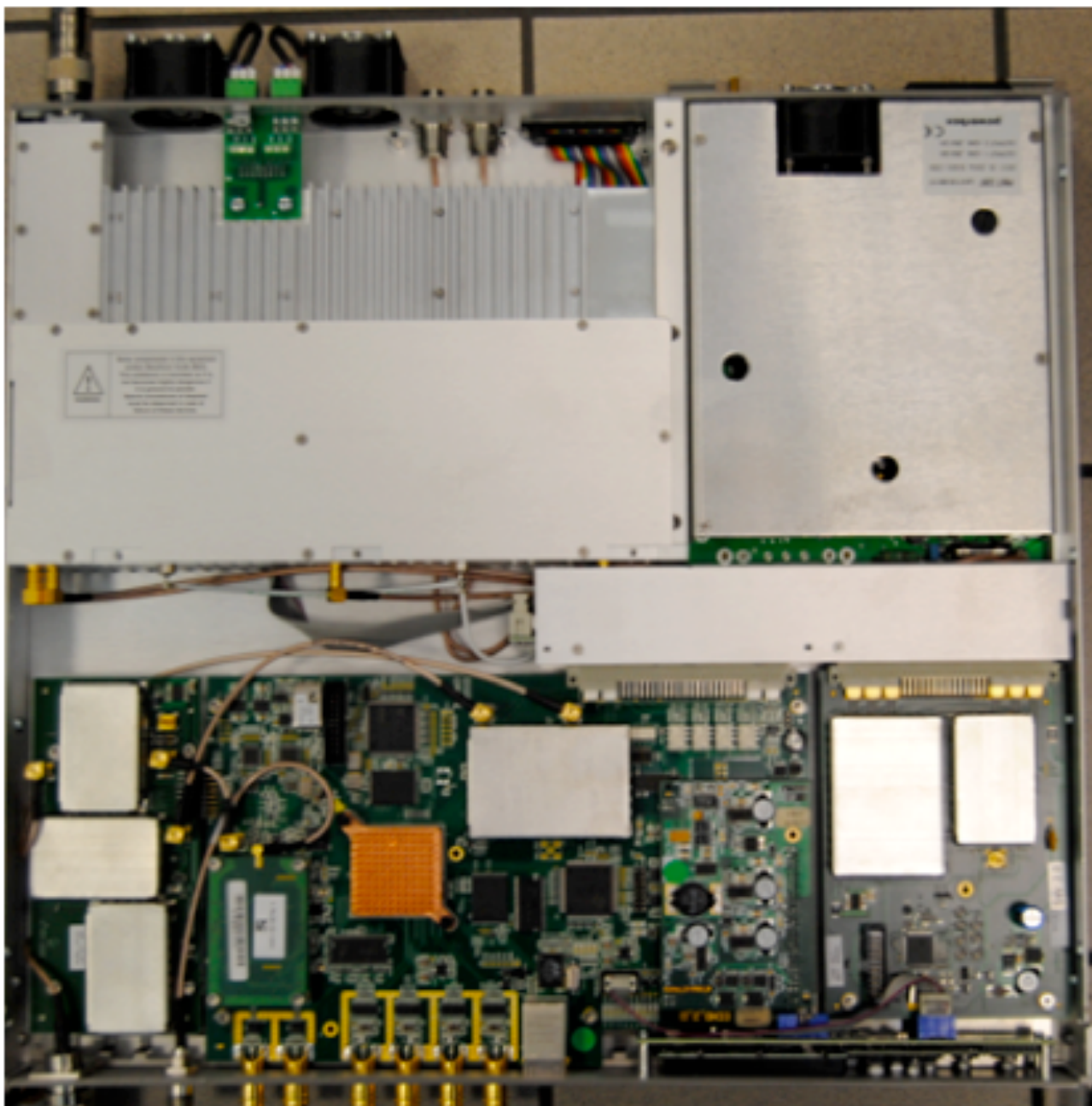
INTERNAL VIEW (OPEN).
