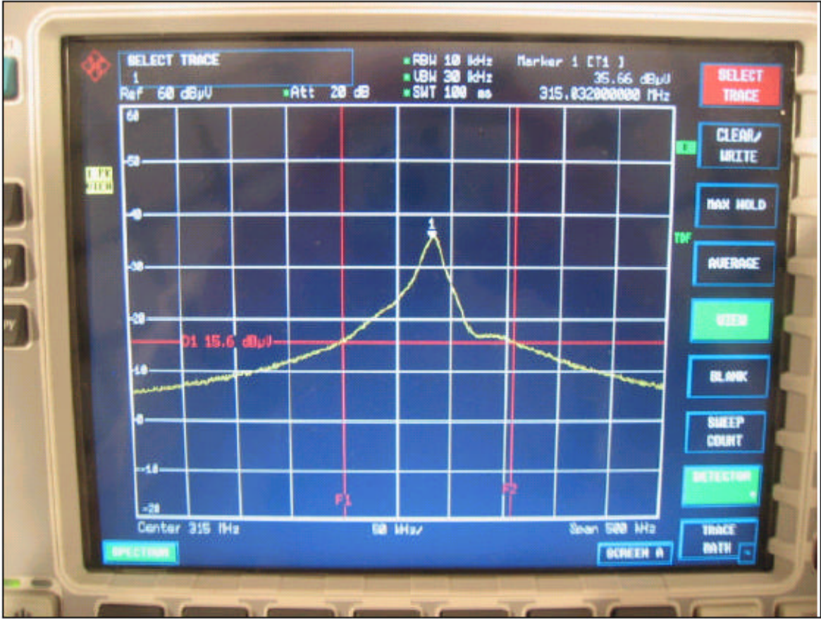
Figure 1: Measured value of the Occupied bandwidth
