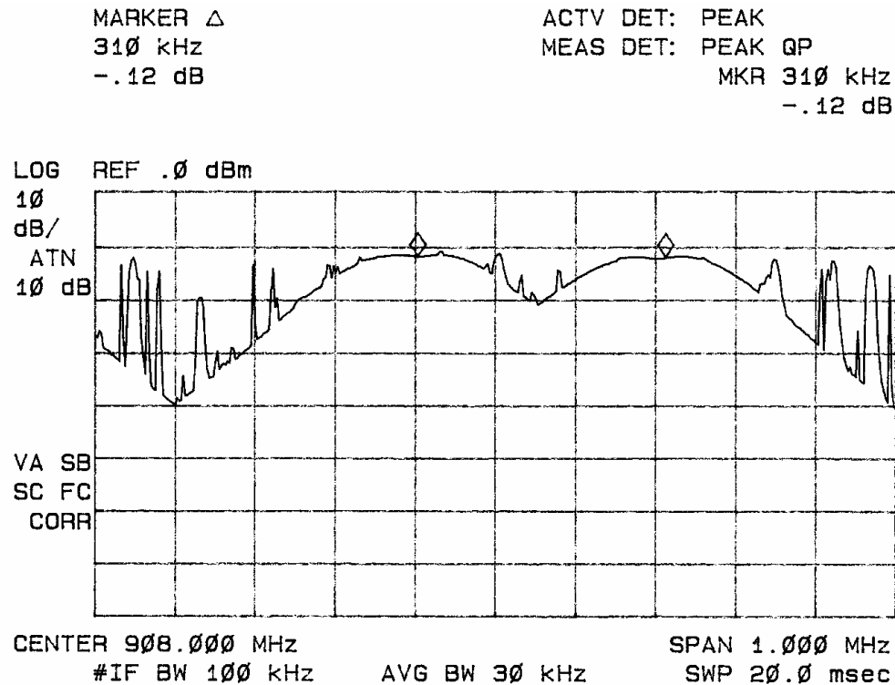
Figure 12 Channel Spacing.
