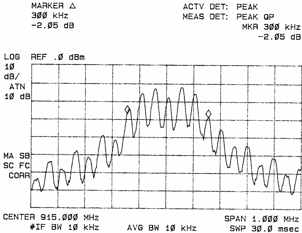
Figure 11 20-dB bandwidth.
