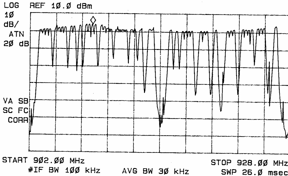
Figure 11 plot showing at least 25 hopping channels.
