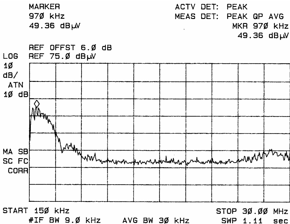
Figure 1 Conducted Emissions Line 1.
