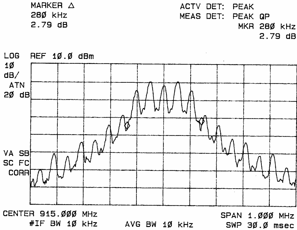
Figure 9 20-dB bandwidth.
