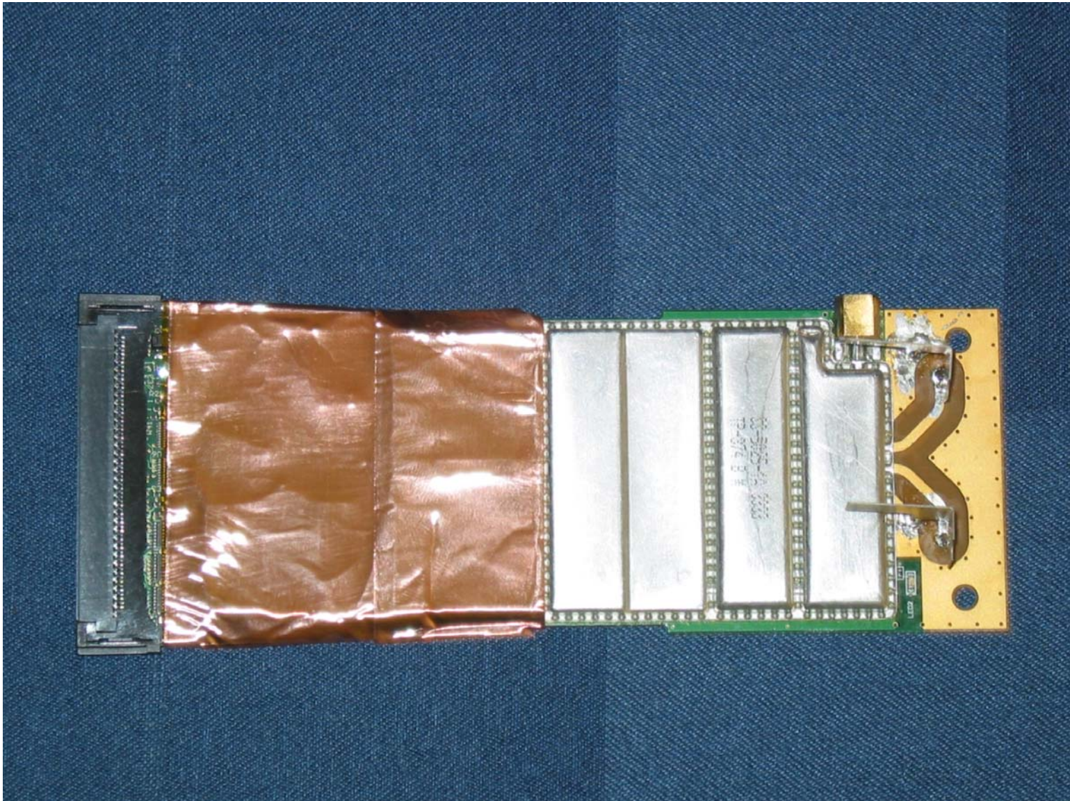
Top View of PWC with Copper Shield on Digital Section
