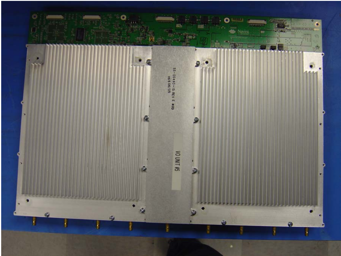
RF Board with Shield (Bottom)
