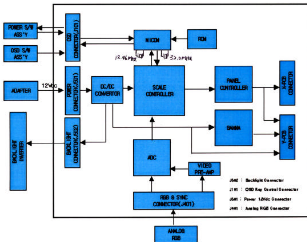
Figure 5 : Block diagram
