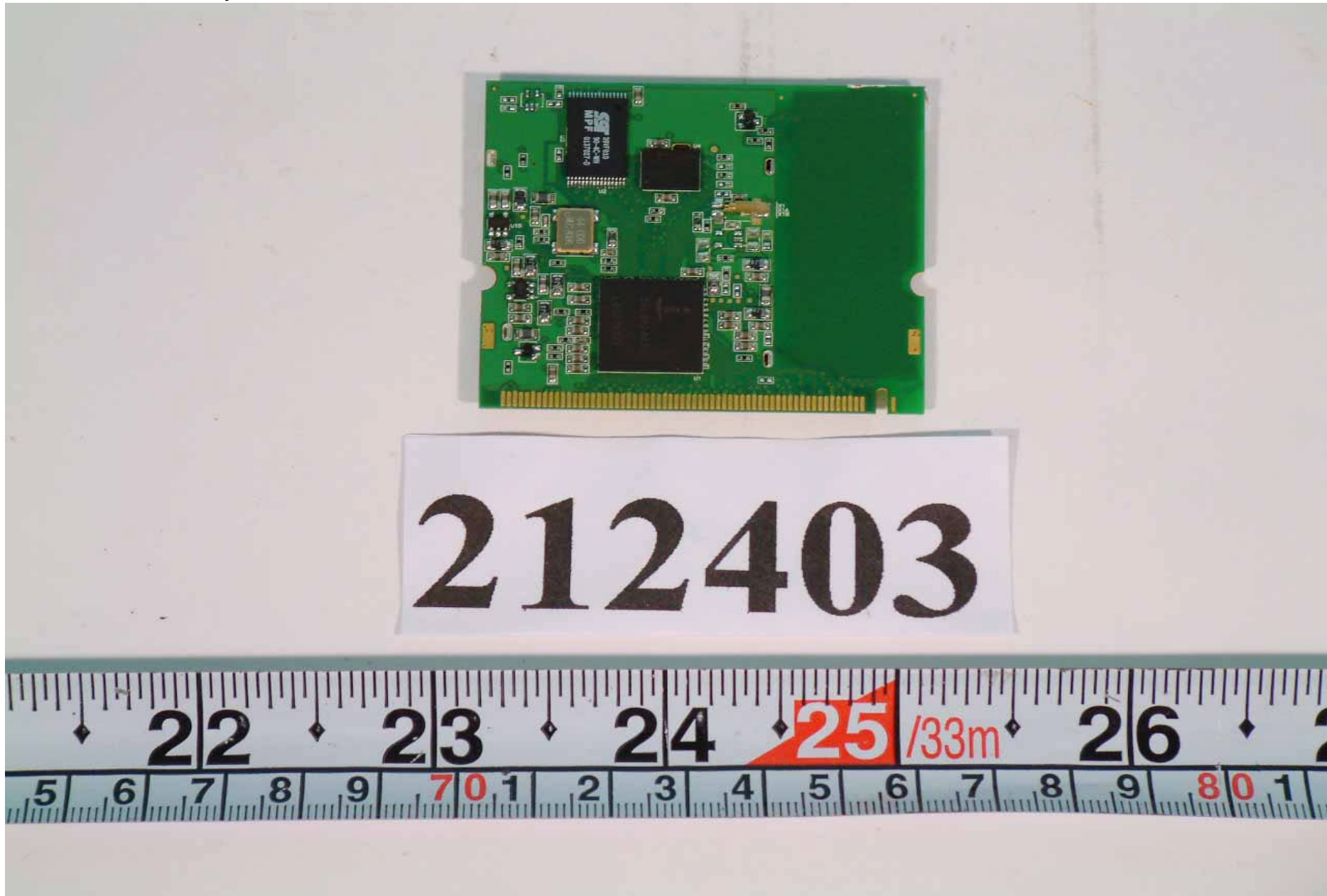
Rear side of 11Mbps Wireless LAN Mini-PCI Card
