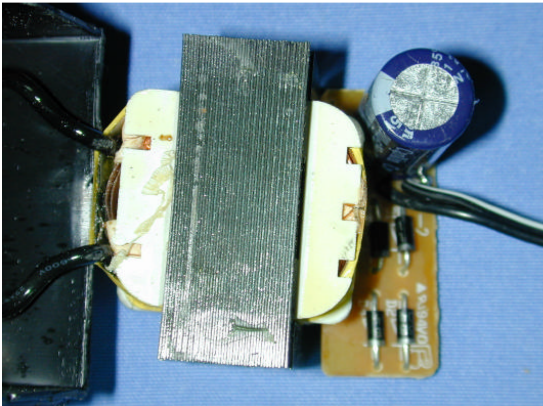
(20) EUT Photo (Mode 1)
