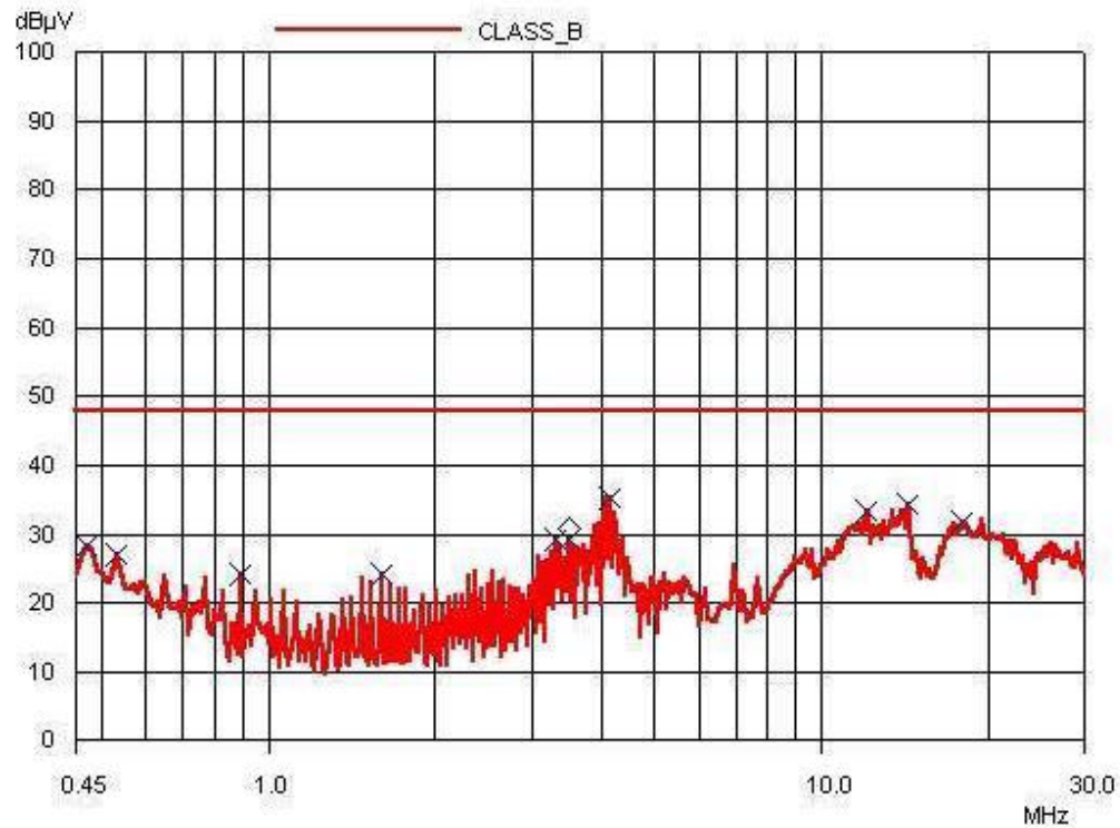
NEUTRAL LINE
