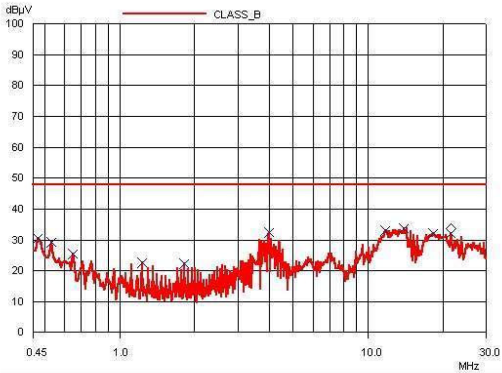
HOT LINE
