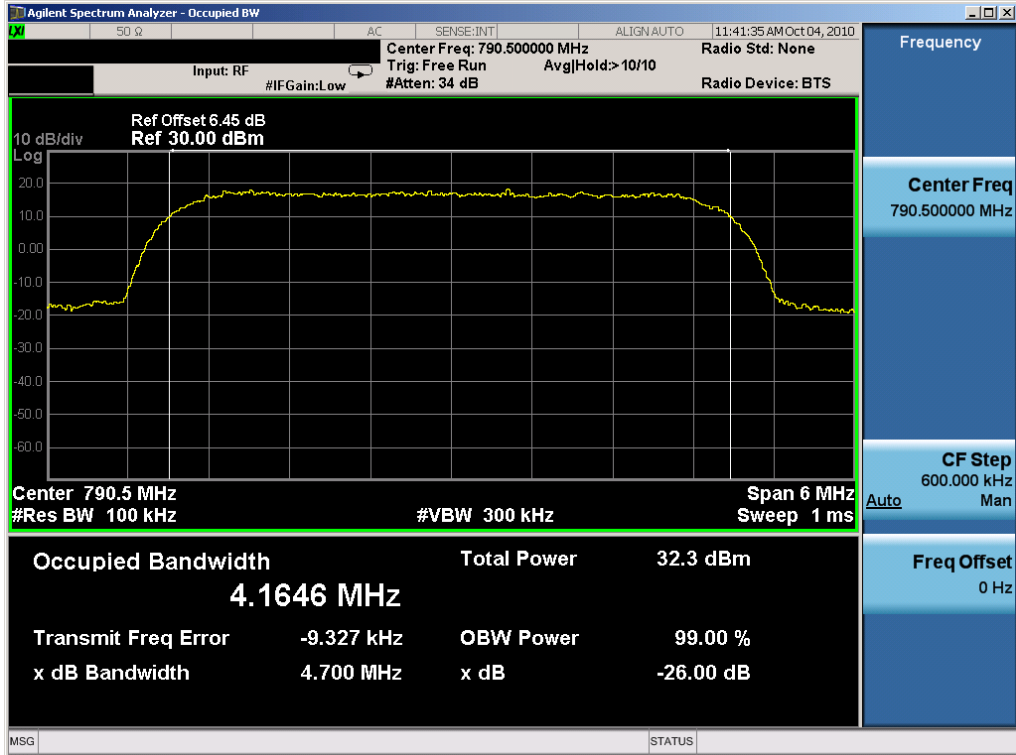
Plot 7-55. Occupied Bandwidth Plot (QPSK, Tx=790.5MHz)
