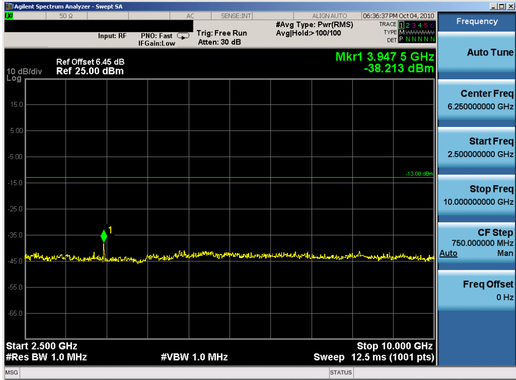
Plot 7-59. Conducted Spurious Plot (64QAM, Tx=790.5MHz)
