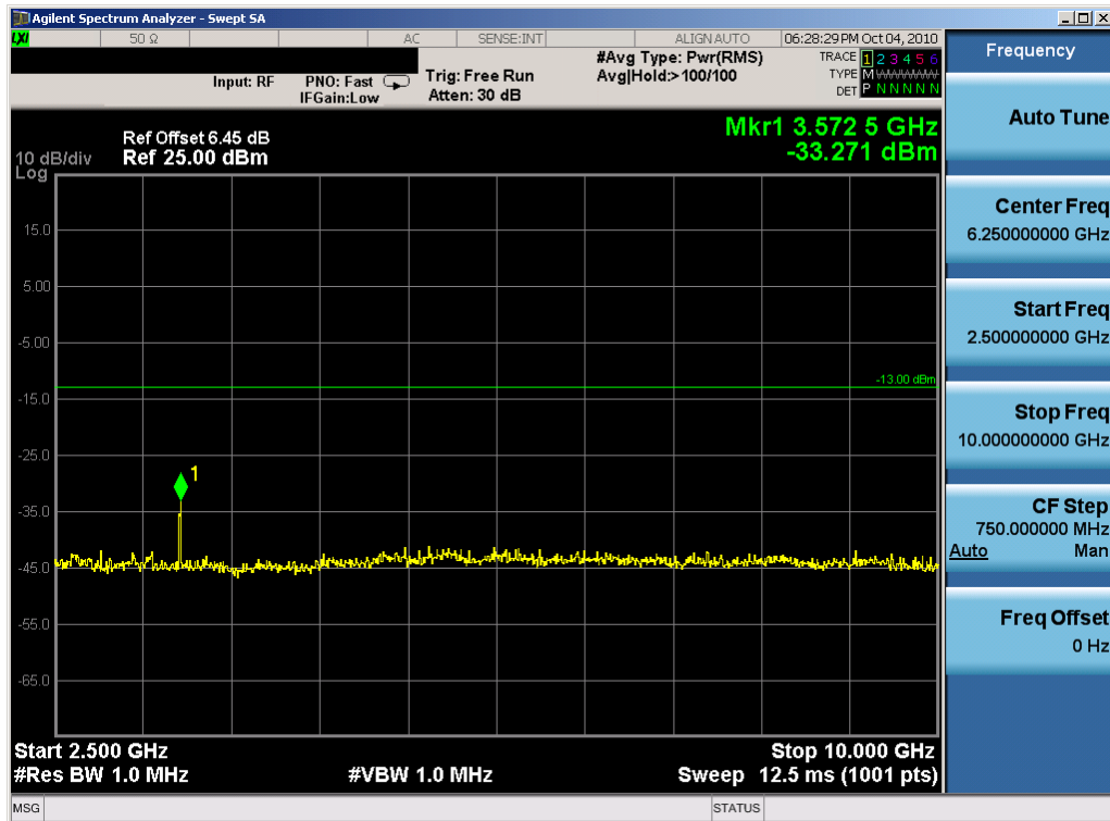
Plot 7-21. Conducted Spurious Plot (64QAM, Tx=713MHz)
