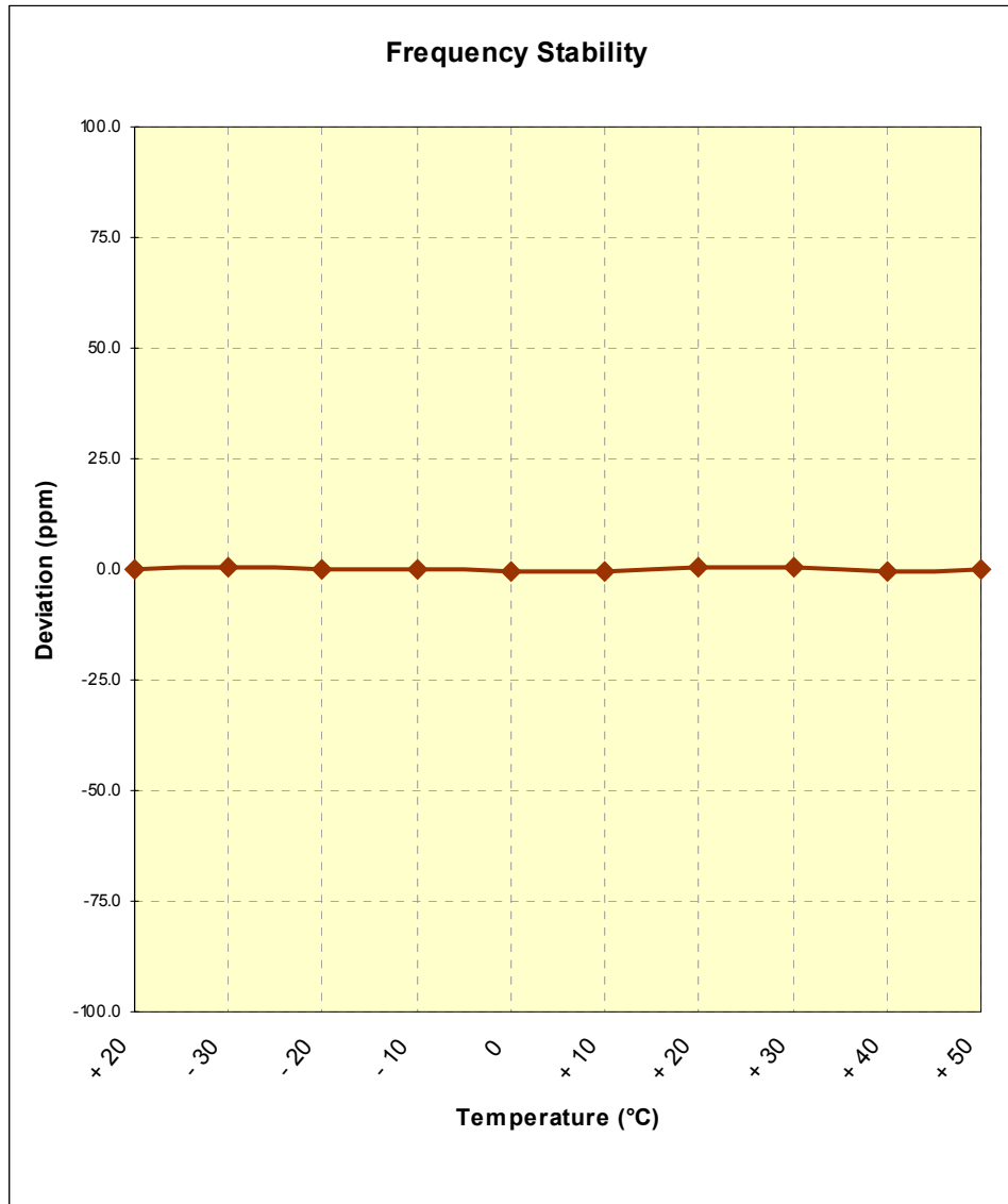
Figure 6-2. Frequency Stability Graph (TD-CDMA Mode Tx=701MHz)
