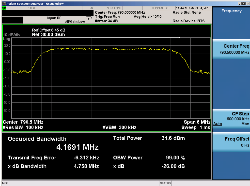
Plot 7-56. Occupied Bandwidth Plot (16QAM, Tx=790.5MHz)
