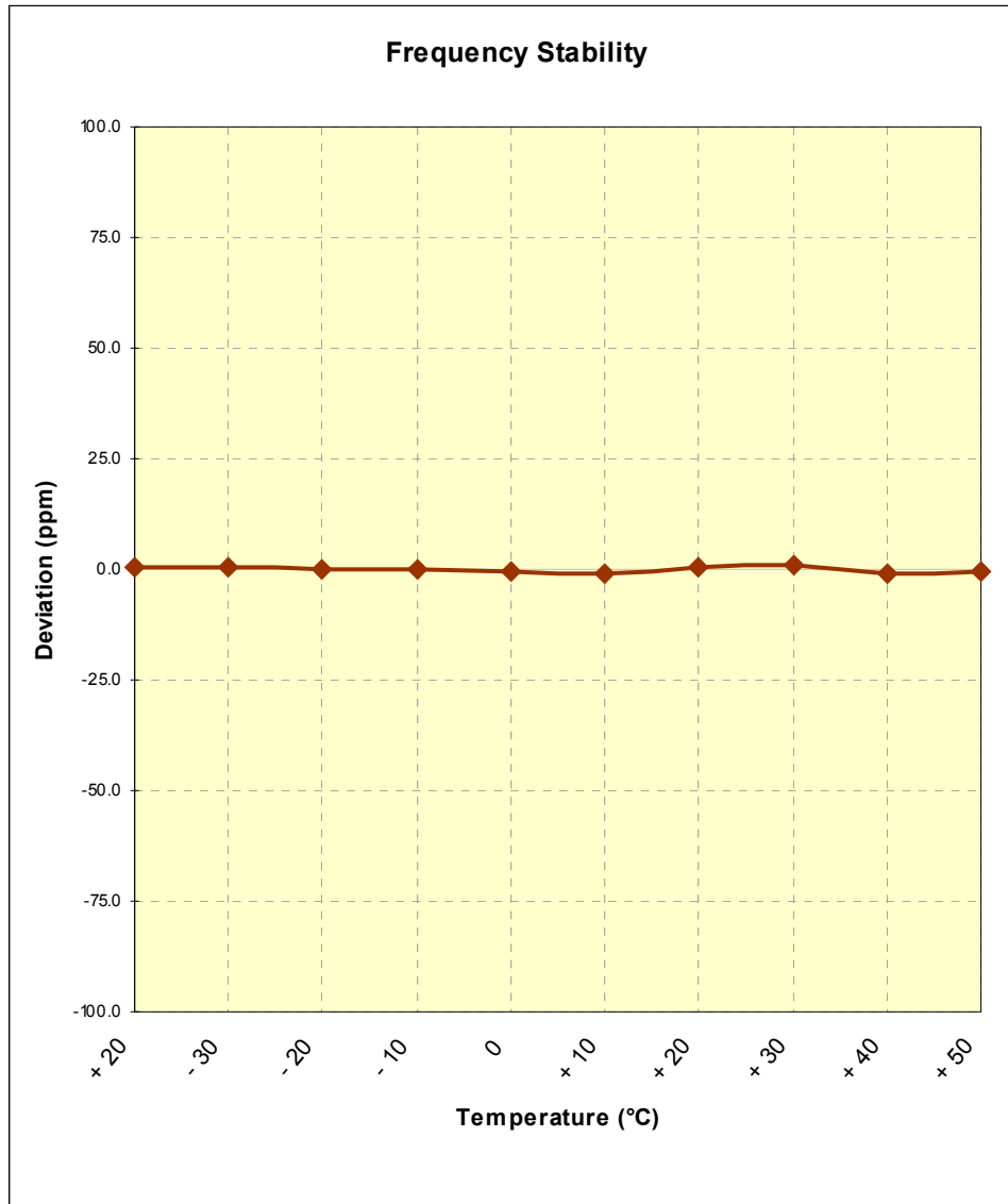
Figure 6-6. Frequency Stability Graph (TD-CDMA Mode Tx=782MHz)
