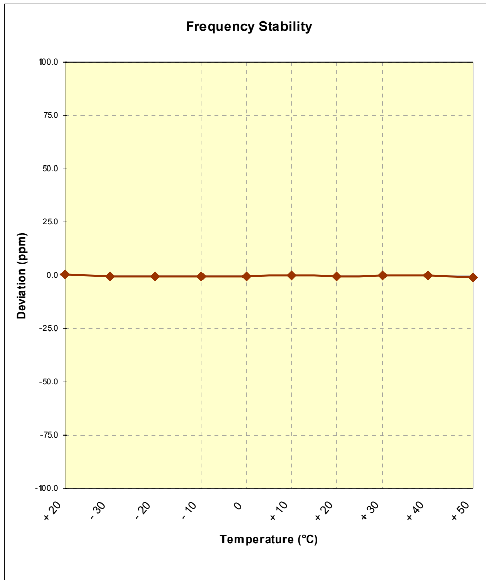
Figure 6-8. Frequency Stability Graph (TD-CDMA Mode Tx=790.5MHz)
