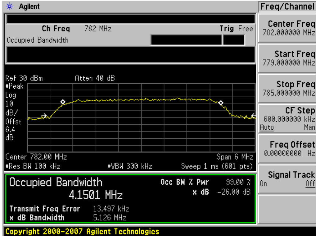
Plot 7-33. Occupied Bandwidth Plot (64QAM, Tx=782 MHz)
