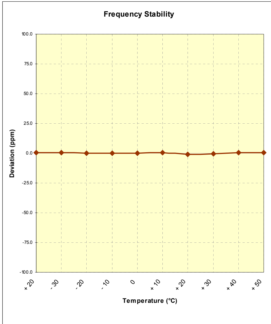
Figure 6-5. Frequency Stability Graph (TD-CDMA Mode Tx=778.5MHz)
