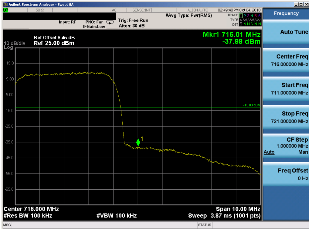
Plot 7-4. Upper Band Edge Plot (QPSK, Tx=713MHz)
