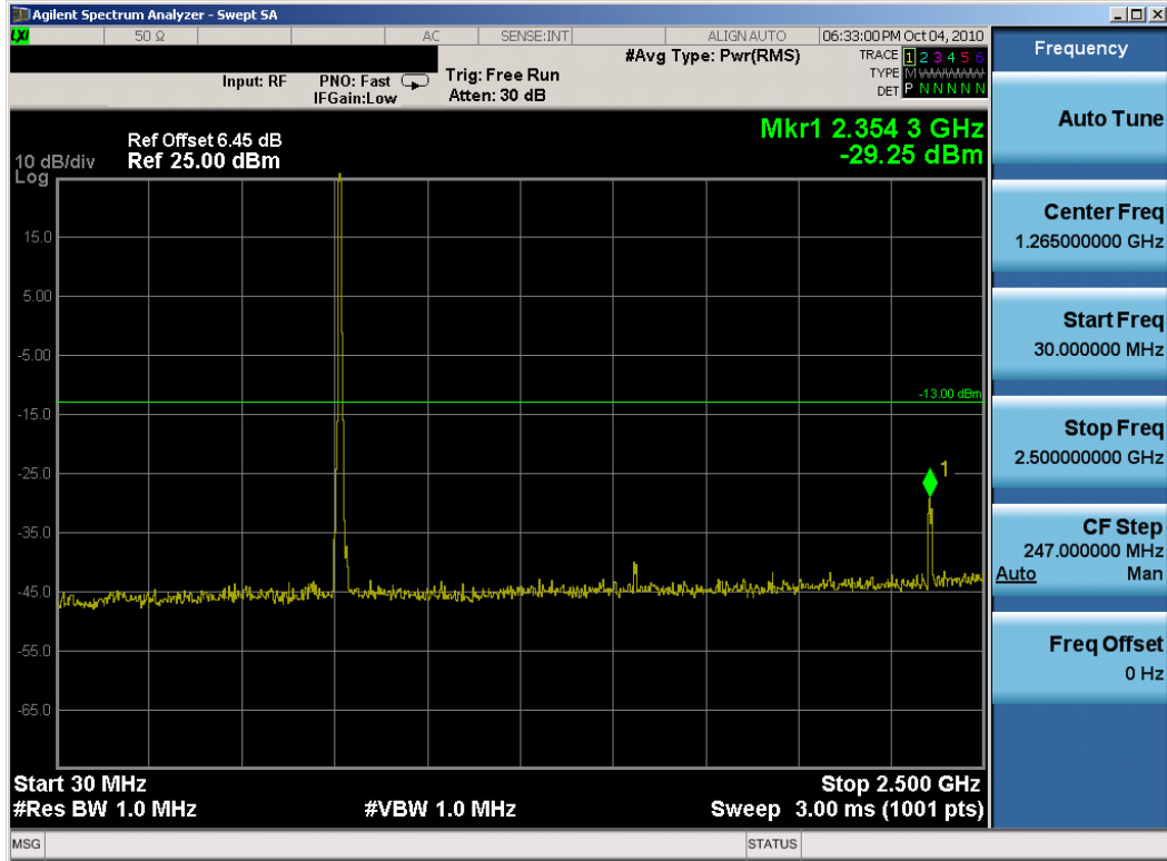
Plot 7-41. Conducted Spurious Plot (64QAM, Tx=785.5MHz)
