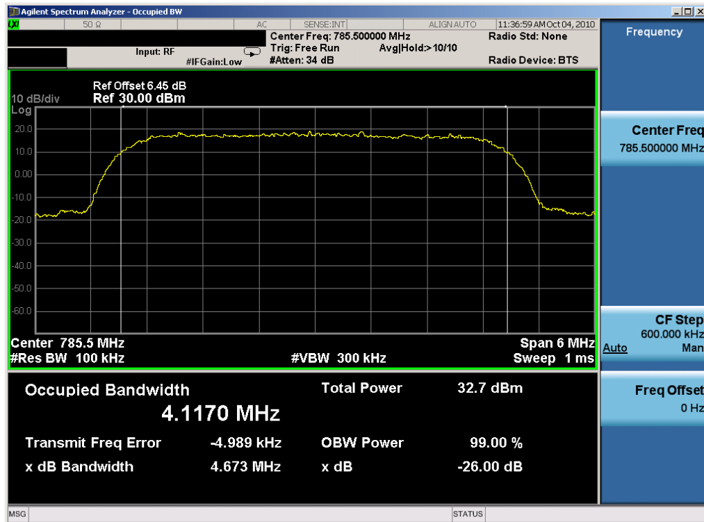
Plot 7-34. Occupied Bandwidth Plot (QPSK, Tx=785.5MHz)
