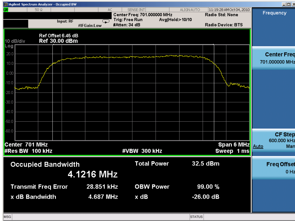
Plot 7-8. Occupied Bandwidth Plot (16QAM, Tx=701MHz)
