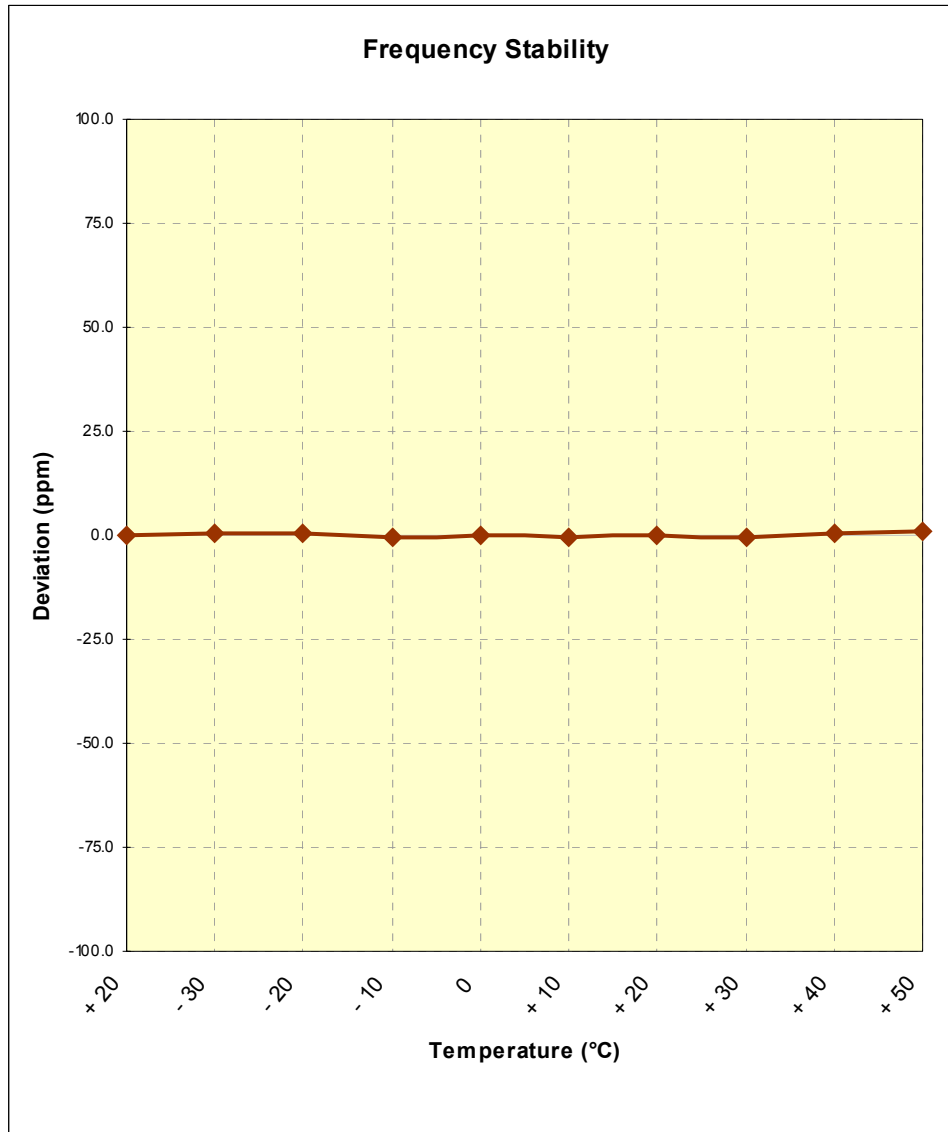
Figure 6-3. Frequency Stability Graph (TD-CDMA Mode Tx=707MHz)
