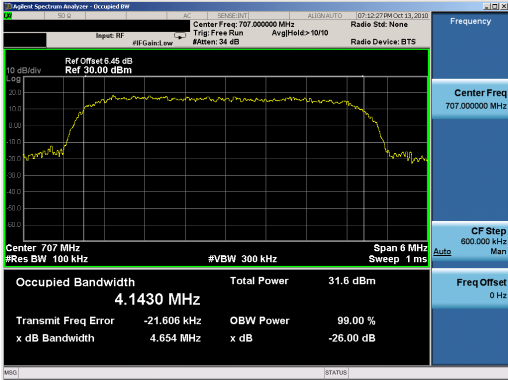
Plot 7-12. Occupied Bandwidth Plot (64QAM, Tx=707MHz)
