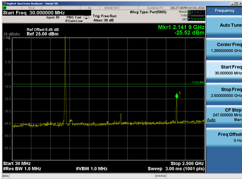
Plot 7-20. Conducted Spurious Plot (64QAM, Tx=713MHz)
