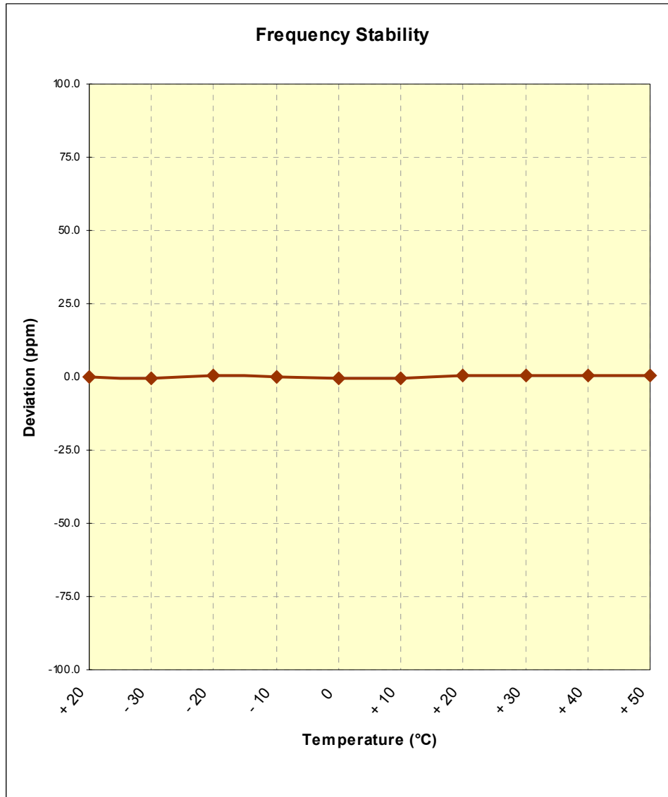
Figure 6-4. Frequency Stability Graph (TD-CDMA Mode - Tx=713MHz)
