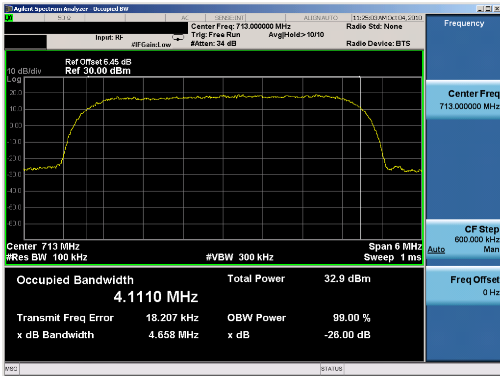
Plot 7-13. Occupied Bandwidth Plot (QPSK, Tx=713MHz)
