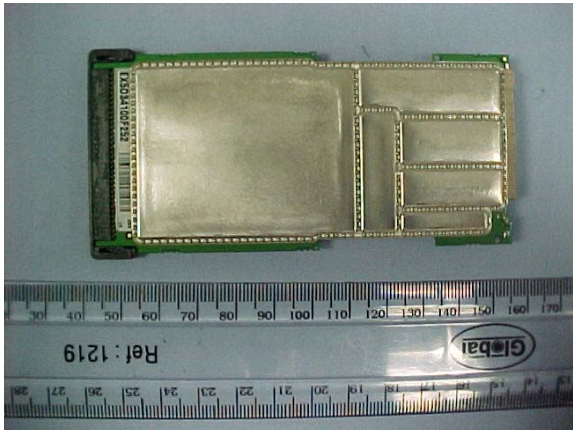
Internal Back View with Antenna Removed
