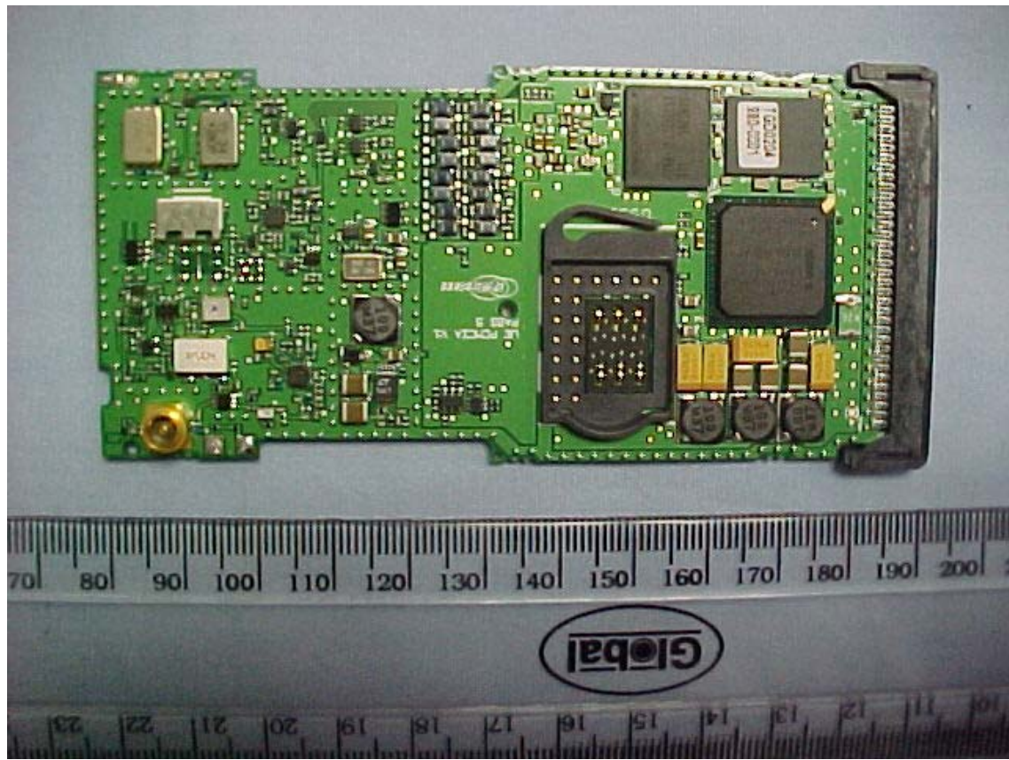
PCB Front View Screens Removed
