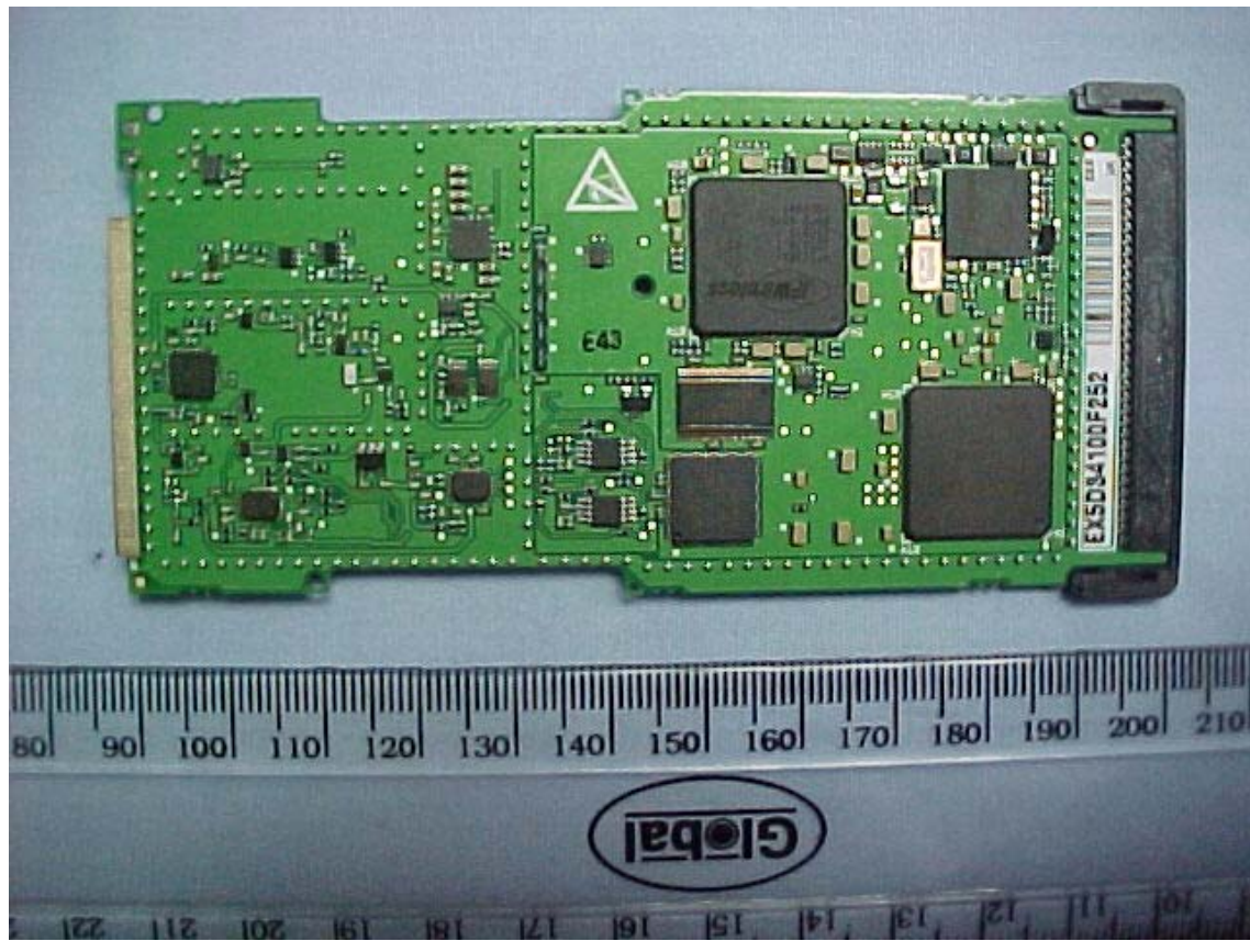
PCB Back View Screens Removed
