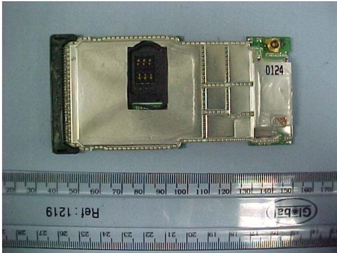
Internal Front View with Antenna Removed
