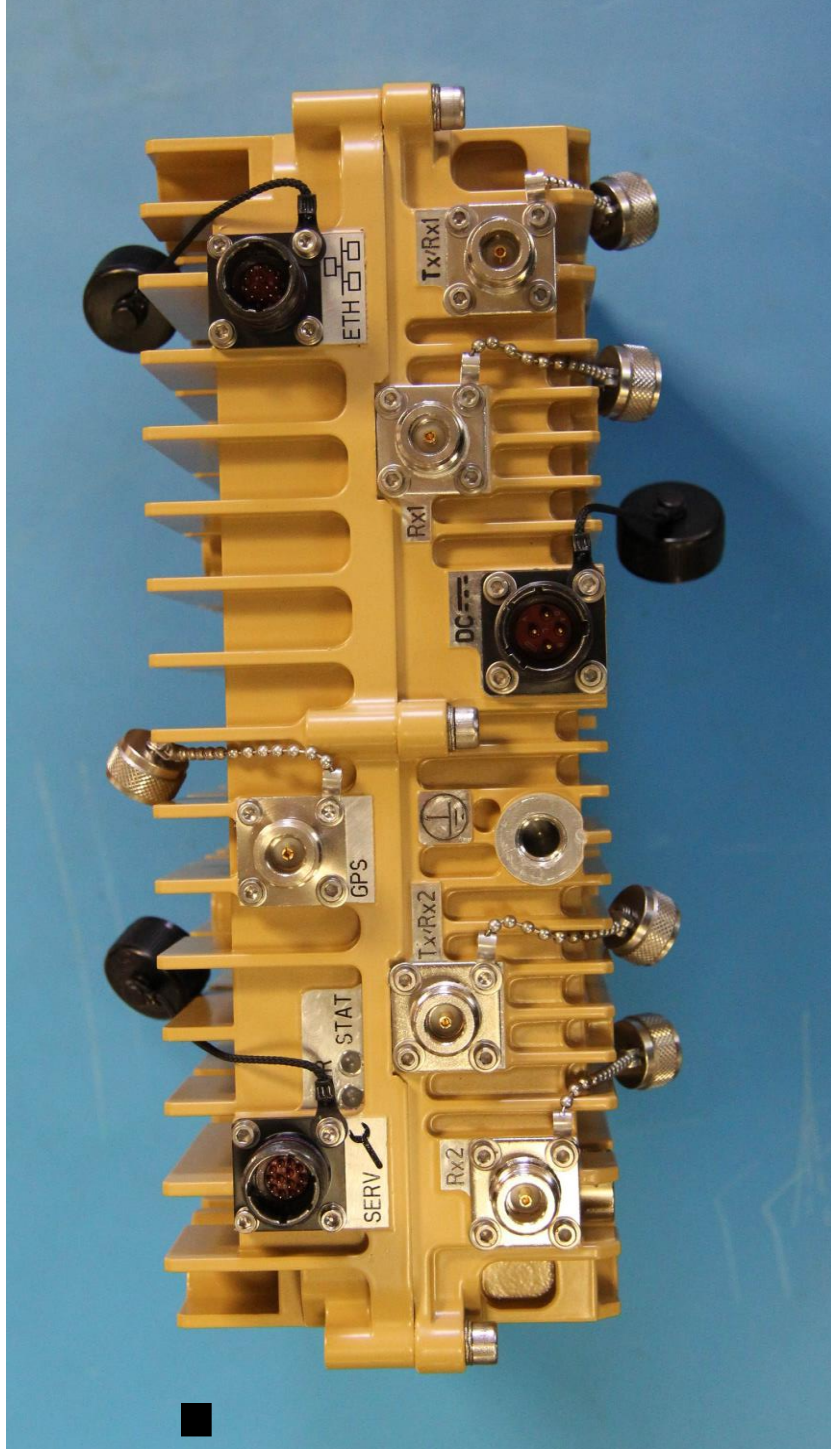
Figure 3: RN2420 External Connectors
