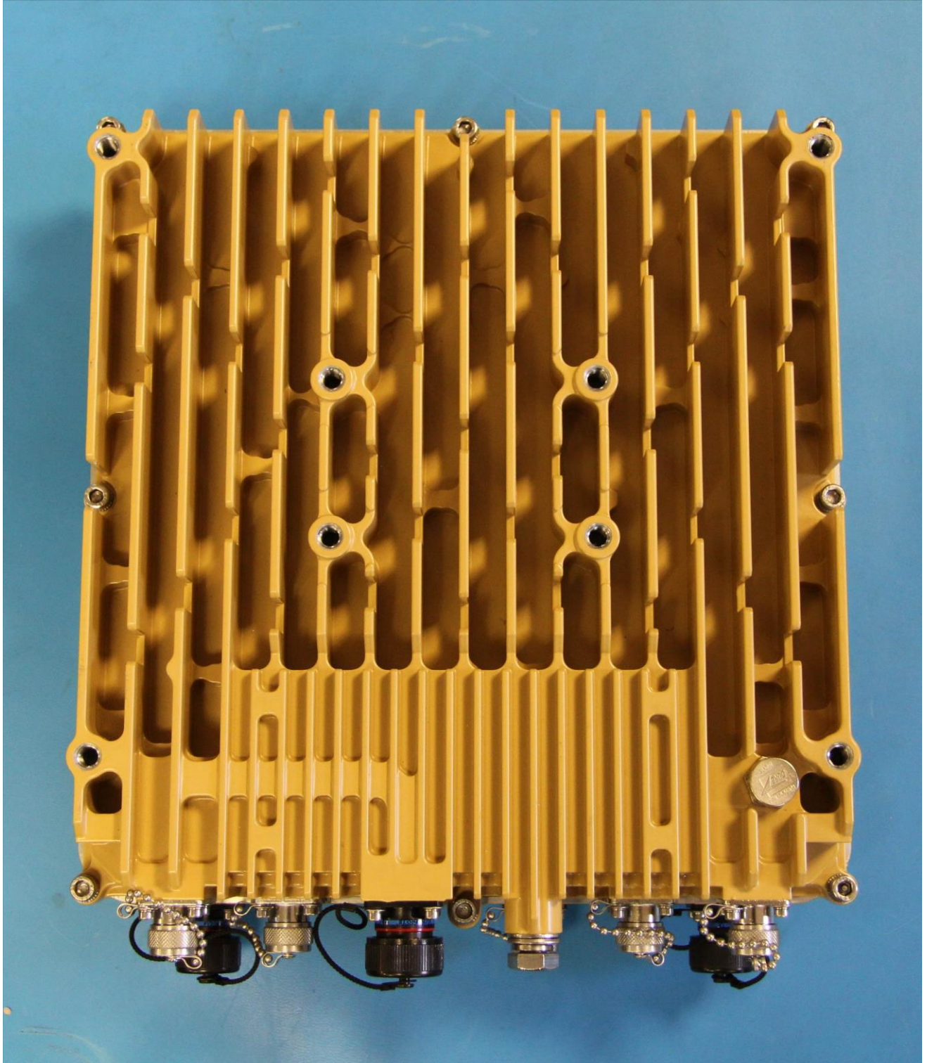
Figure 2: RN2420 eNodeB Rear View
