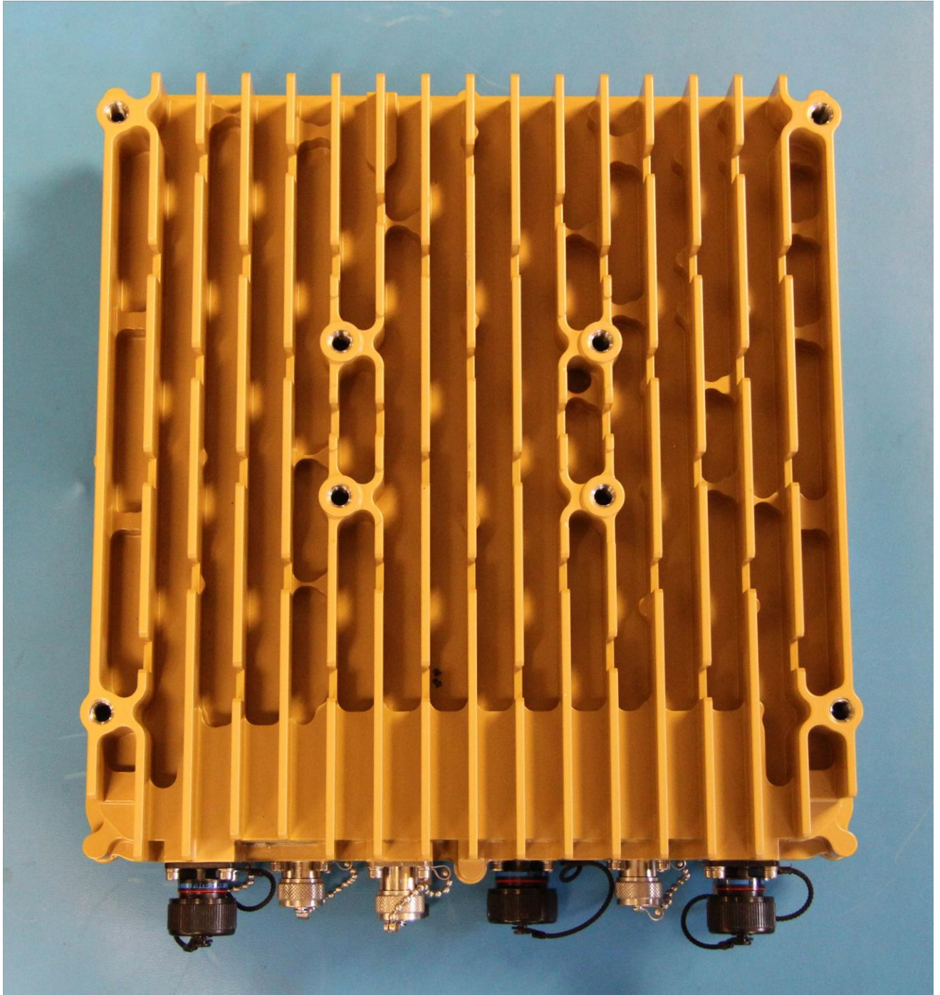
Figure 1: RN2420 eNodeB Front View
