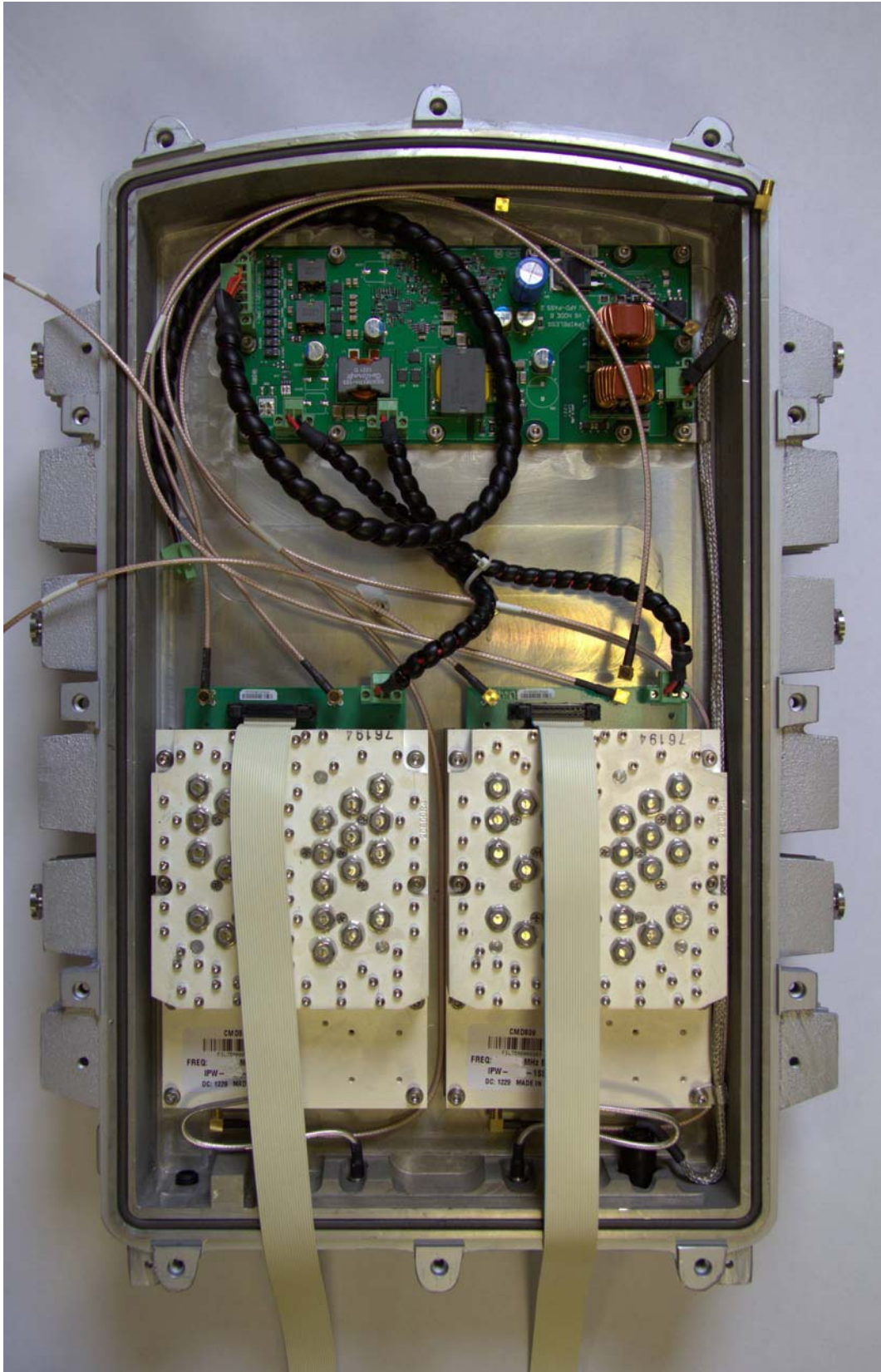
Figure 2: Rear Casting Internal View
