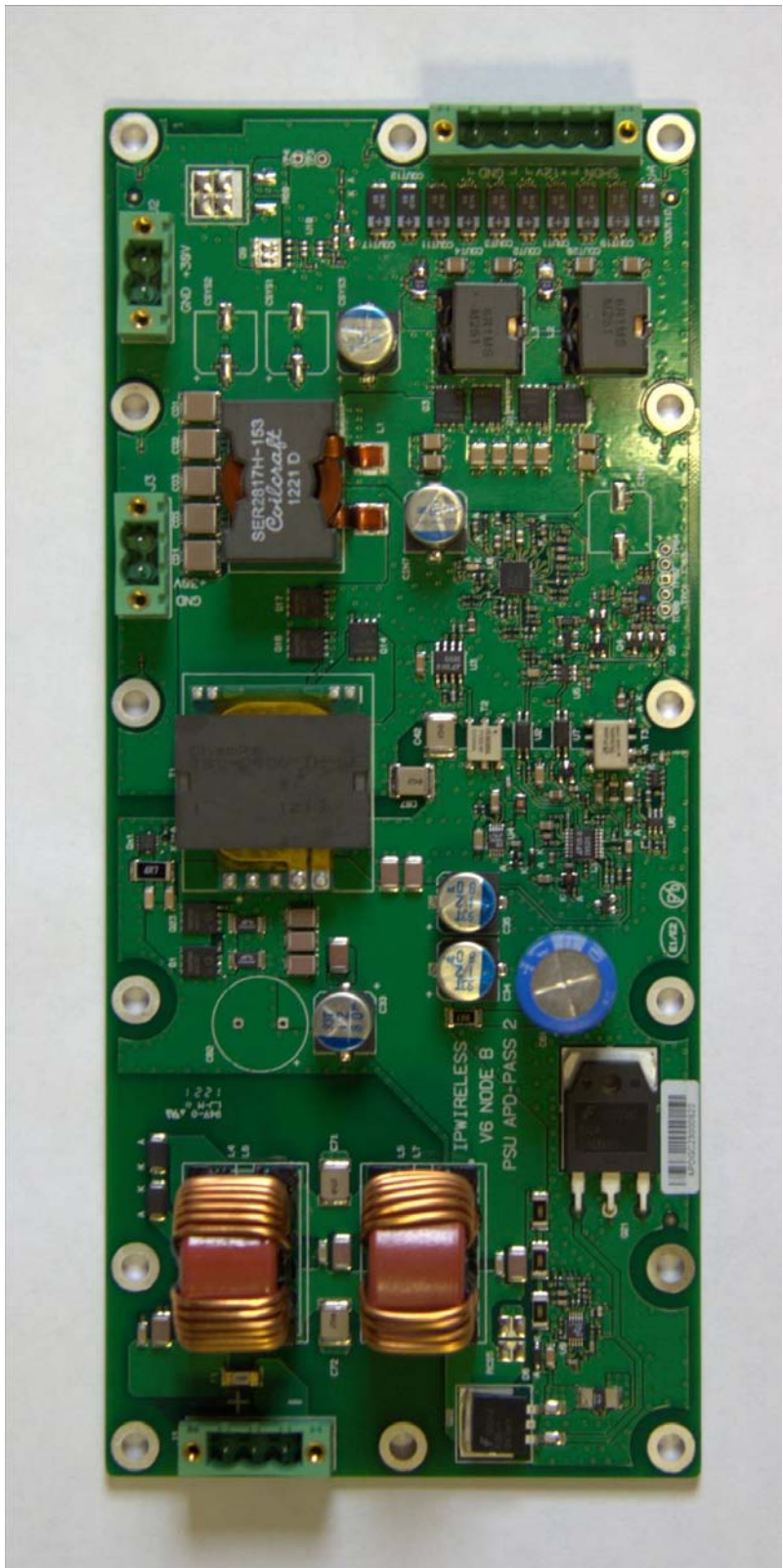
Figure 7: Power Supply Top View
