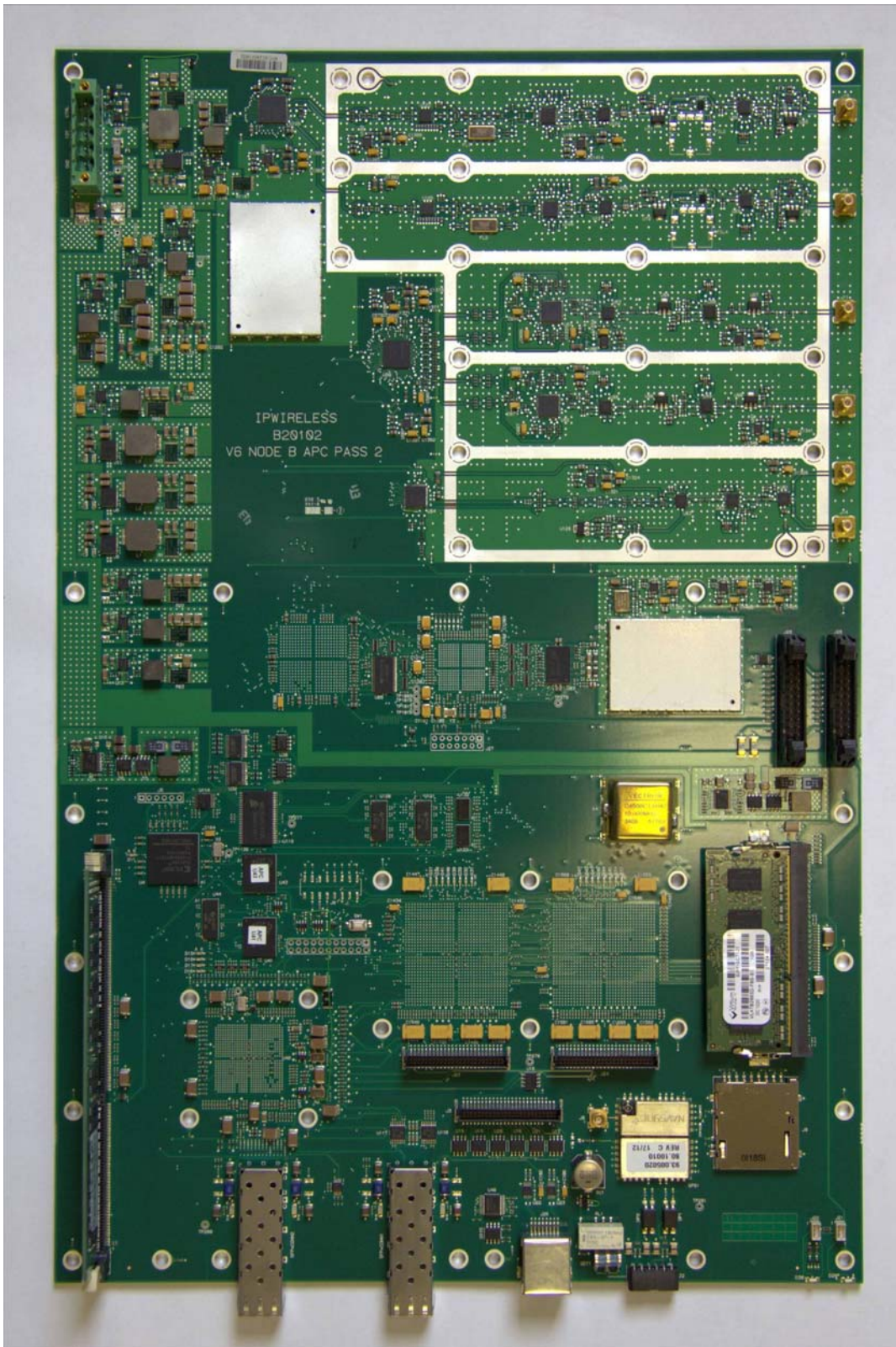
Figure 3: Main Board Front View
