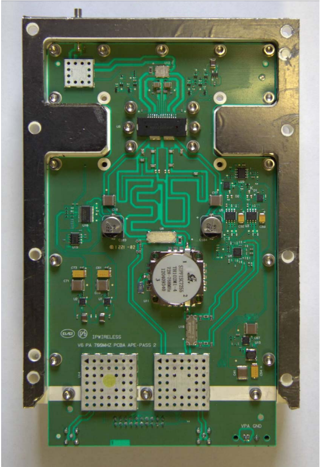
Figure 6: Power Amplifier Board Fitted in Filter
