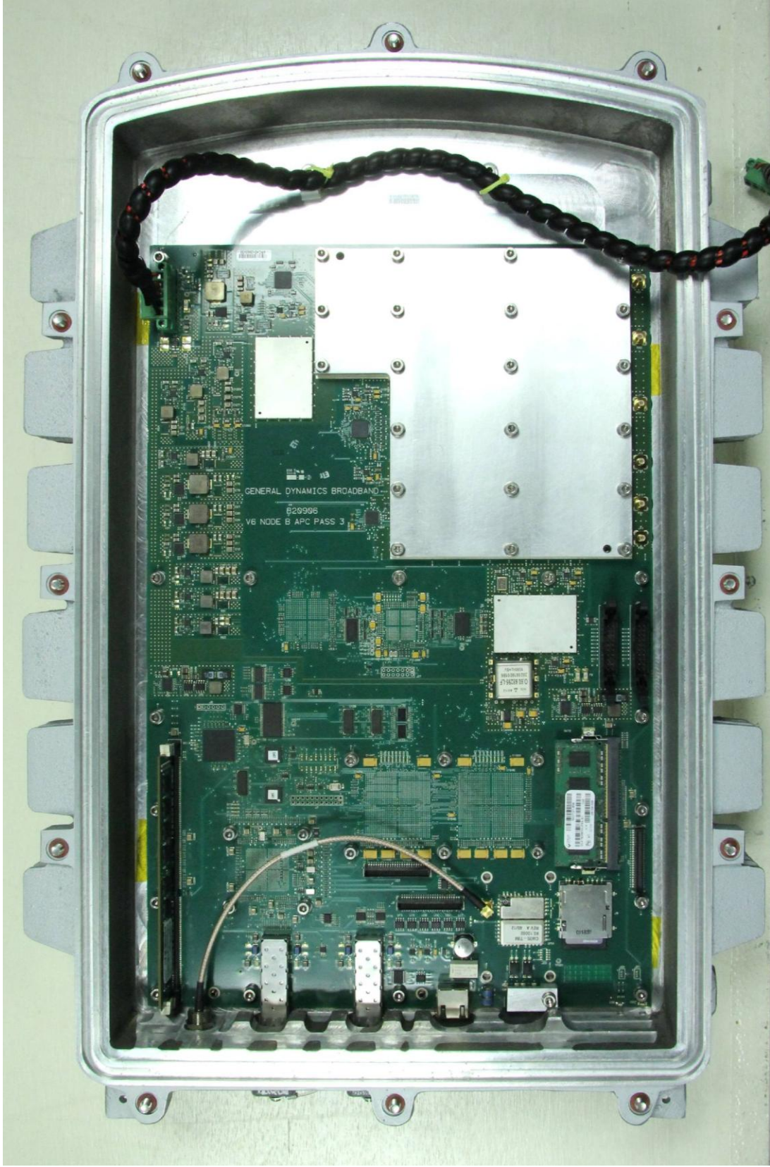
Figure 1: Front Casting Internal View
