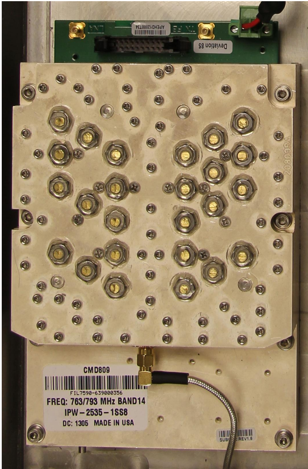
Figure 5: Power Amplifier and Filter Assembly Top View
