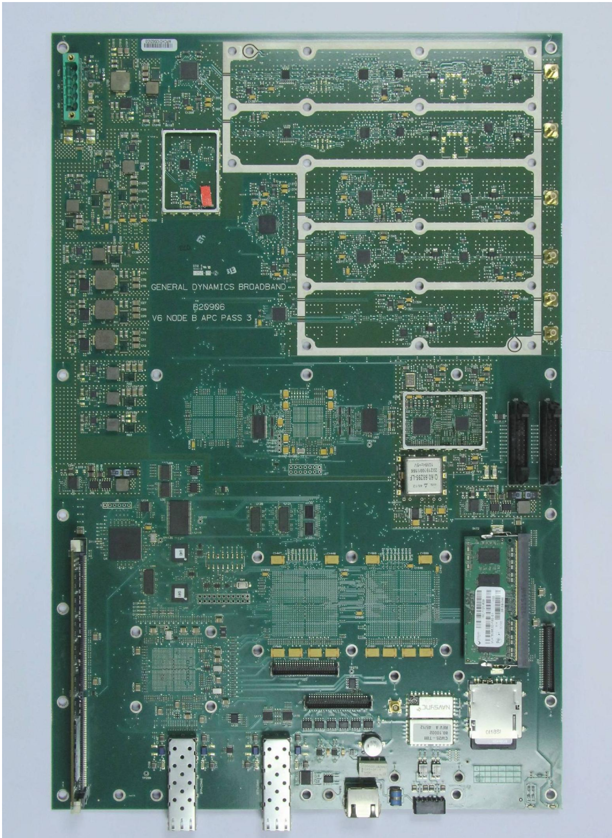
Figure 3: Main Board Front View
