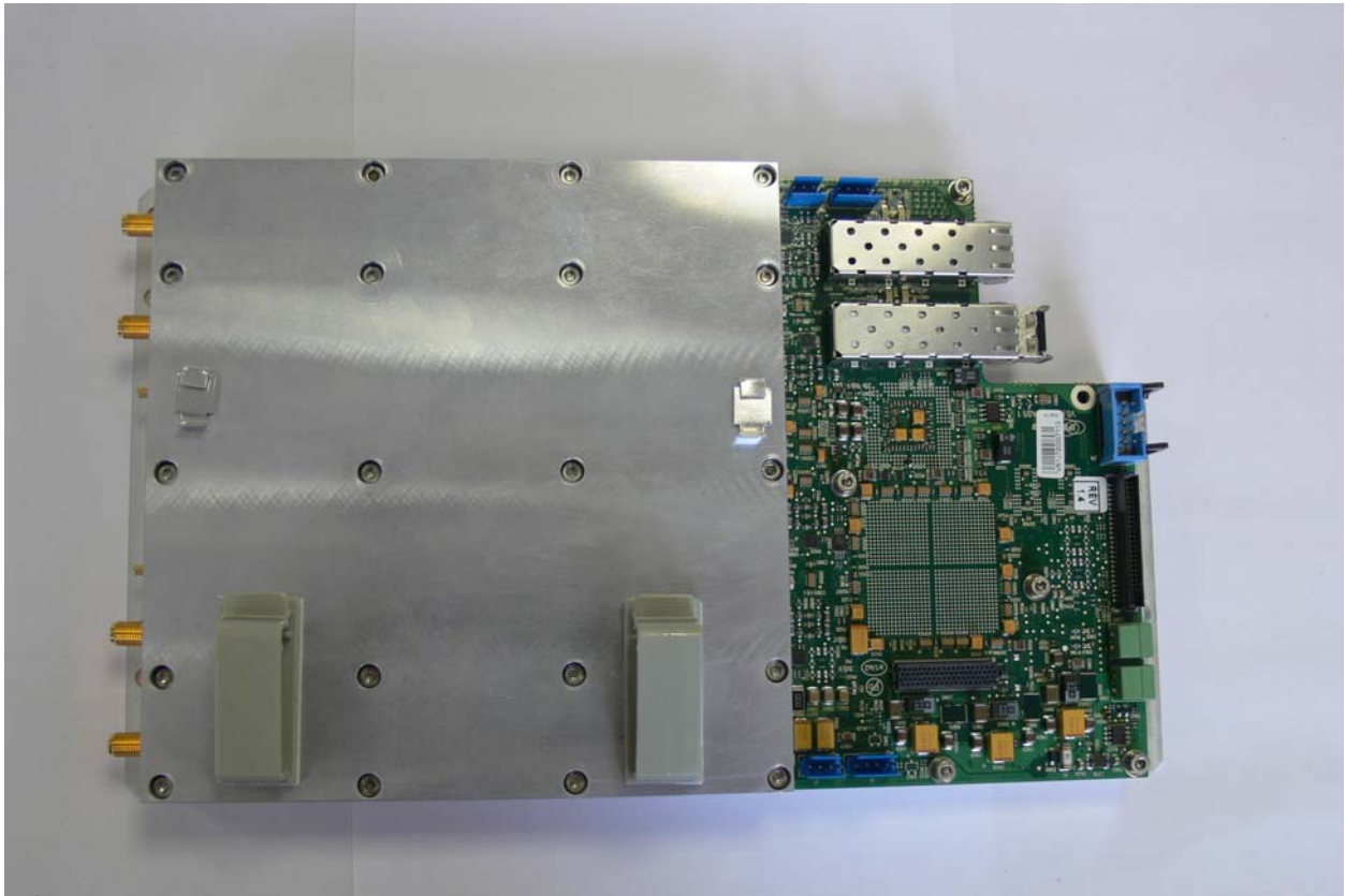
Figure 3: Radio Card In Clamshell
