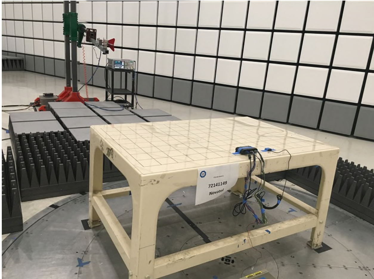
FCC Part 15B Radiated Emissions Test Setup (above 1GHz)
