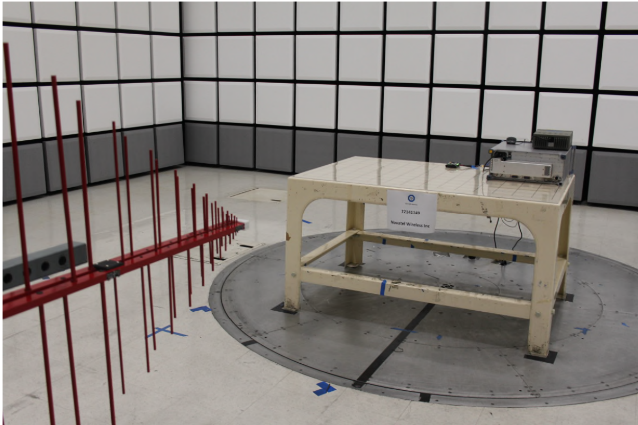
Radiated Emissions Test Setup – Tx Mode (below 1GHz)
