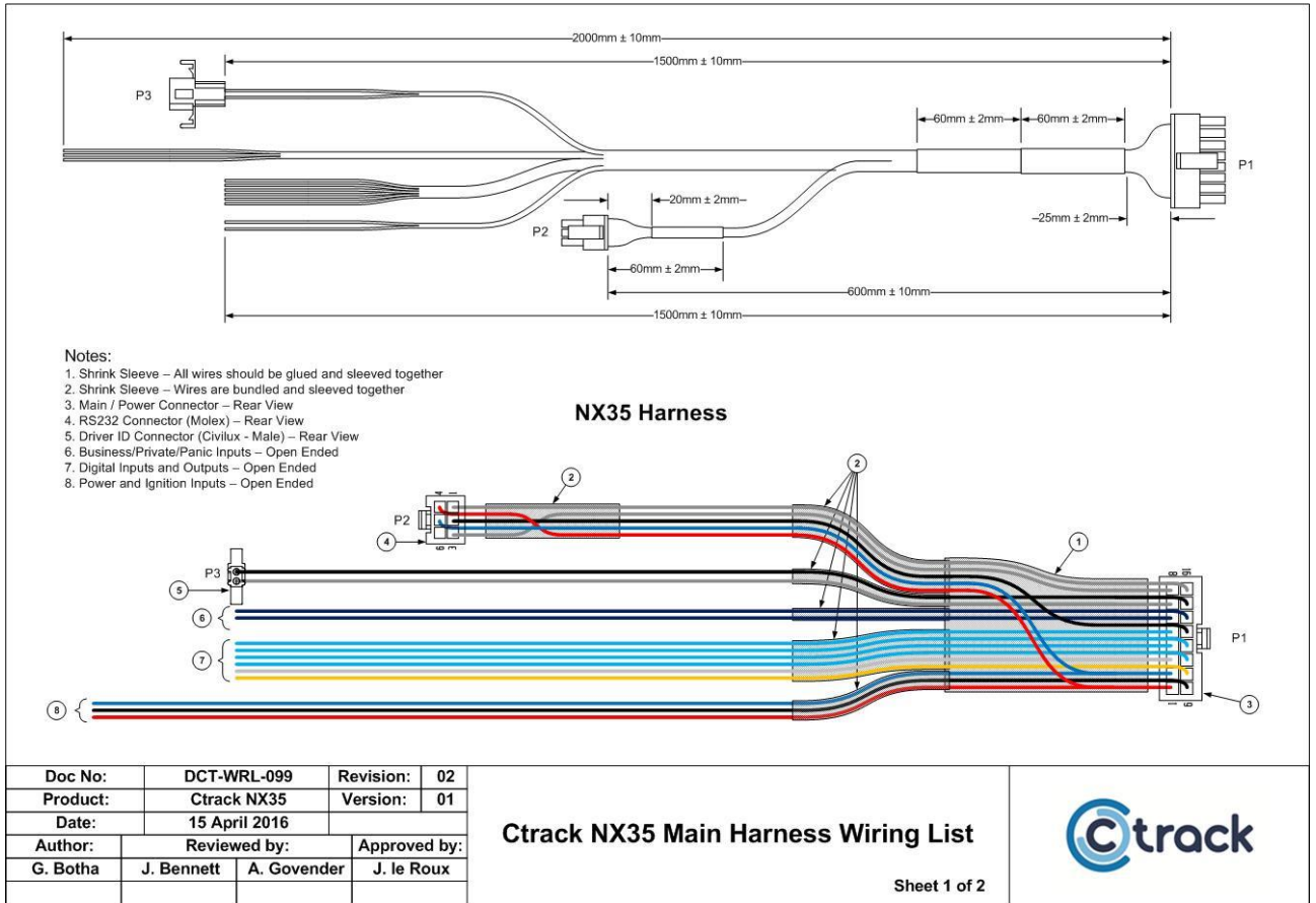
FIGURE 2 - MAIN HARNESS
