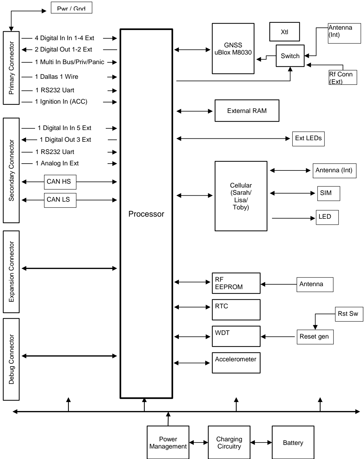
FIGURE 1 - BLOCK DIAGRAM
