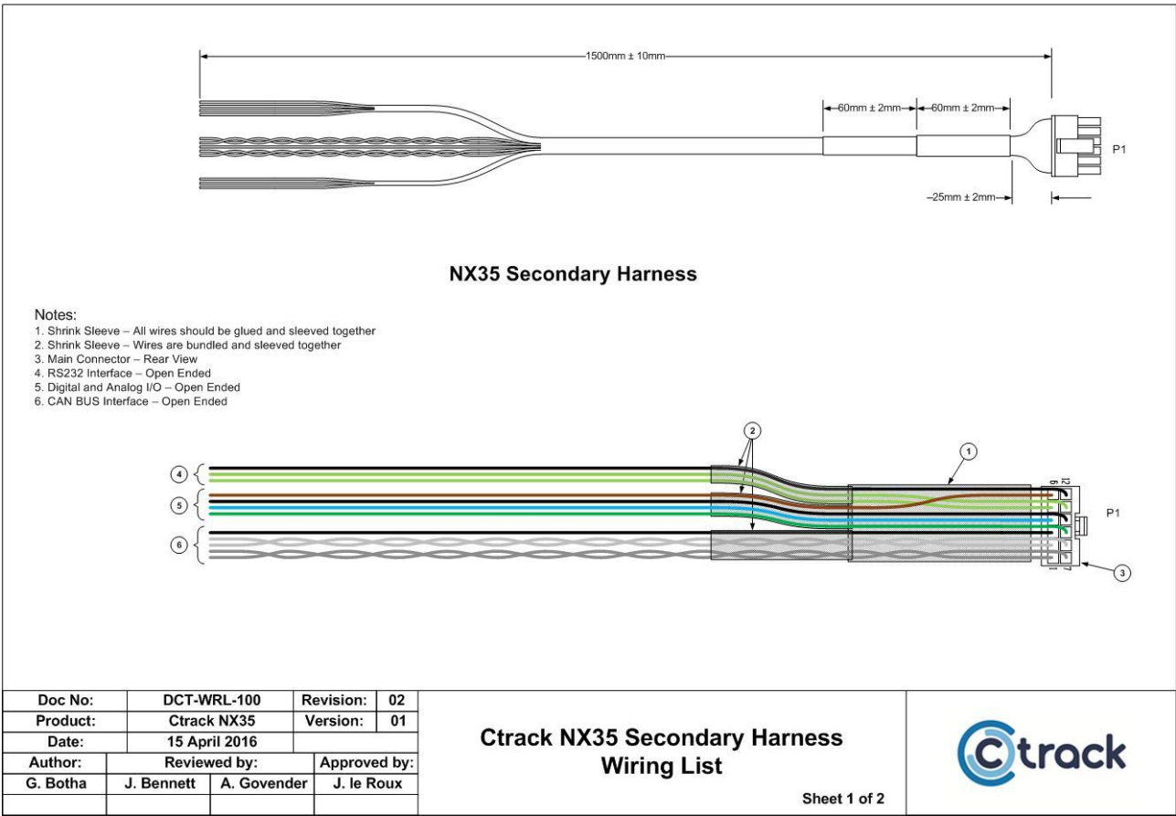
FIGURE 4 - SECONDARY HARNESS
