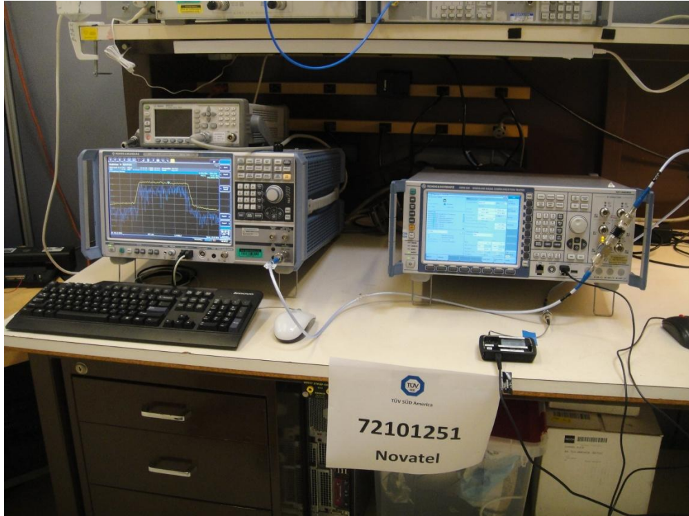
Antenna Conducted Port Measurement
