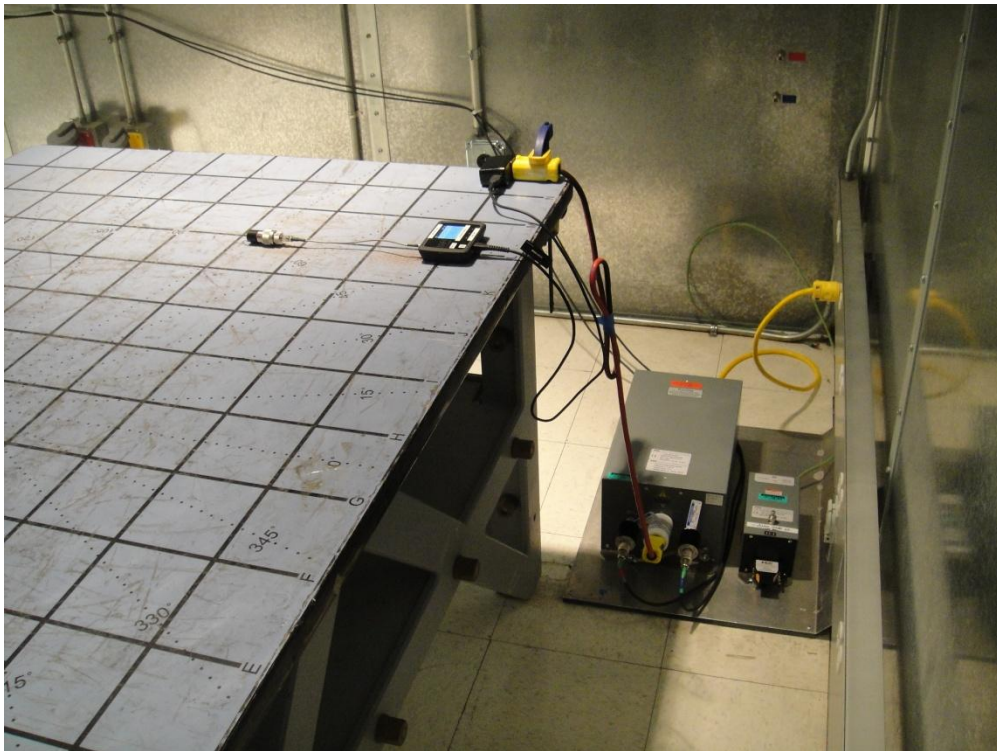
Conducted Emission Measurement (Front and Rear)
