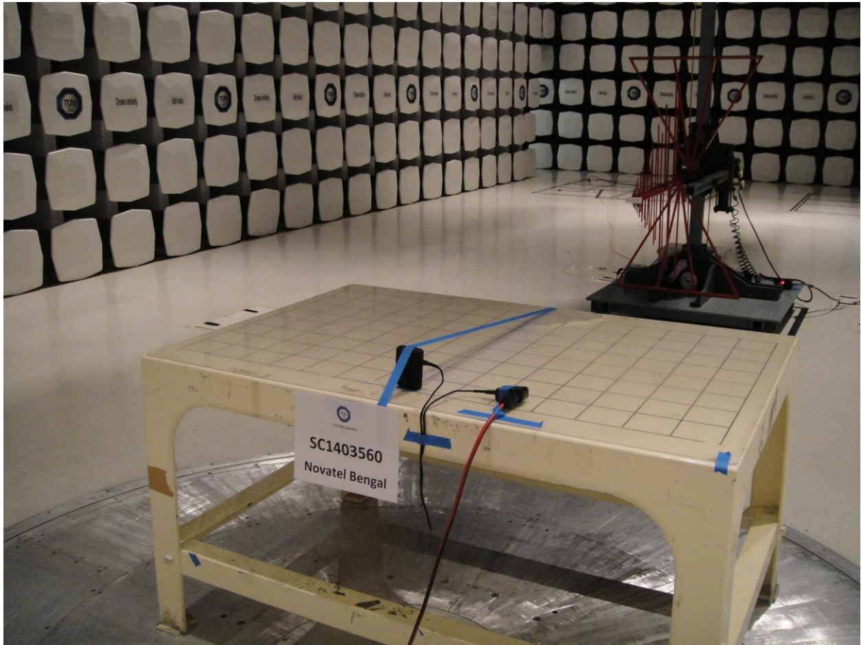
Radiated Emission test below 1GHz (Back)
