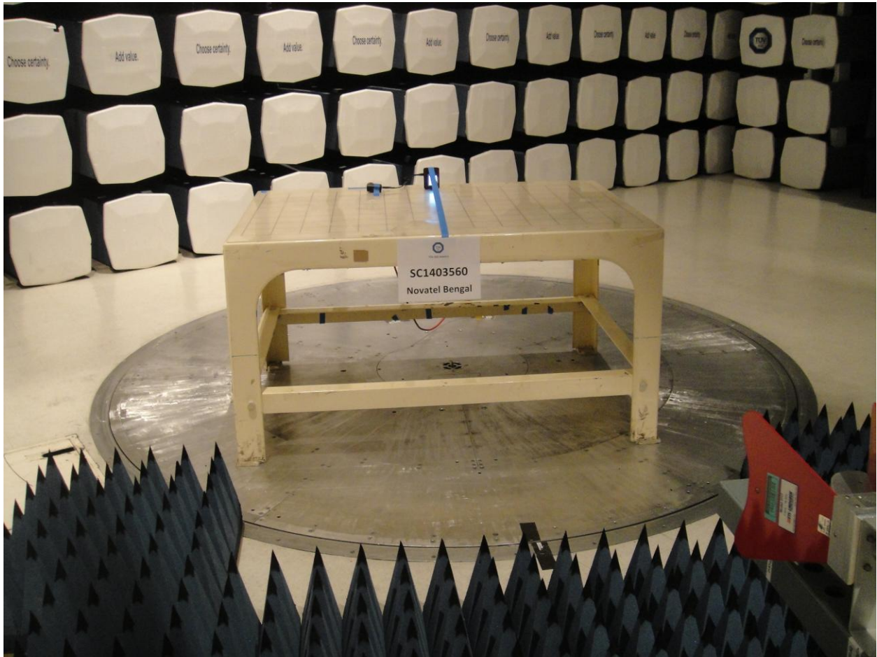
Radiated Emission test above 1GHz (Front)
