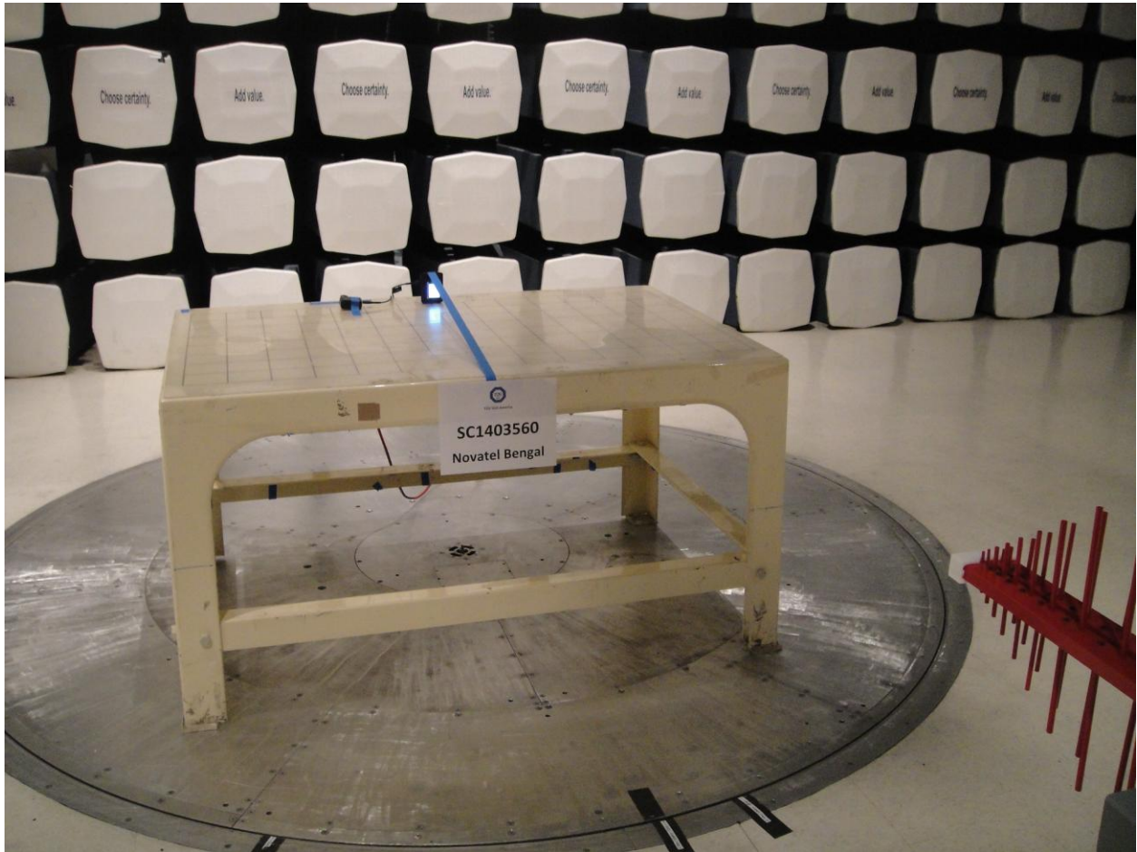
Radiated Emission test below 1GHz (Front)
