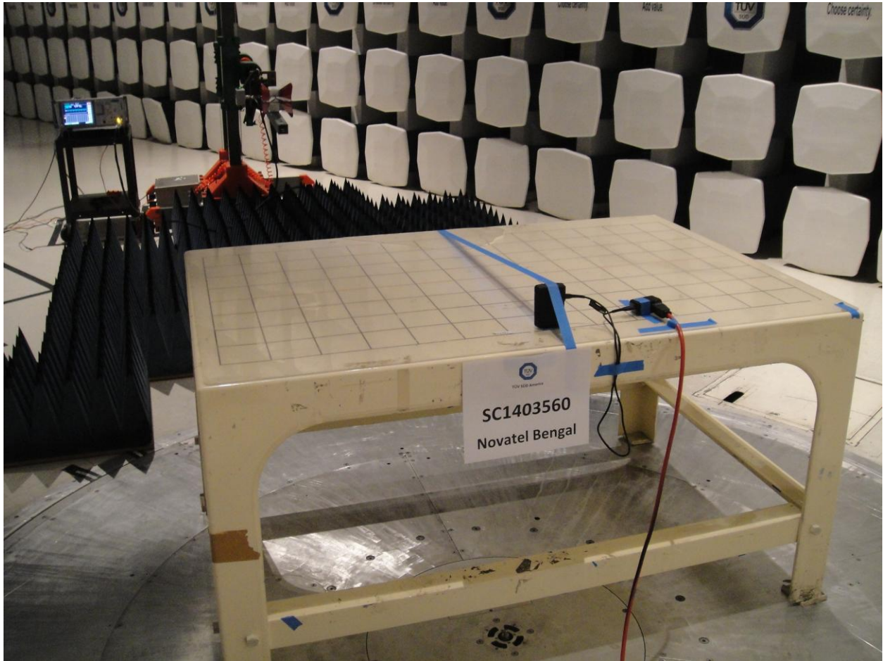
Radiated Emission test above 1GHz (back)
