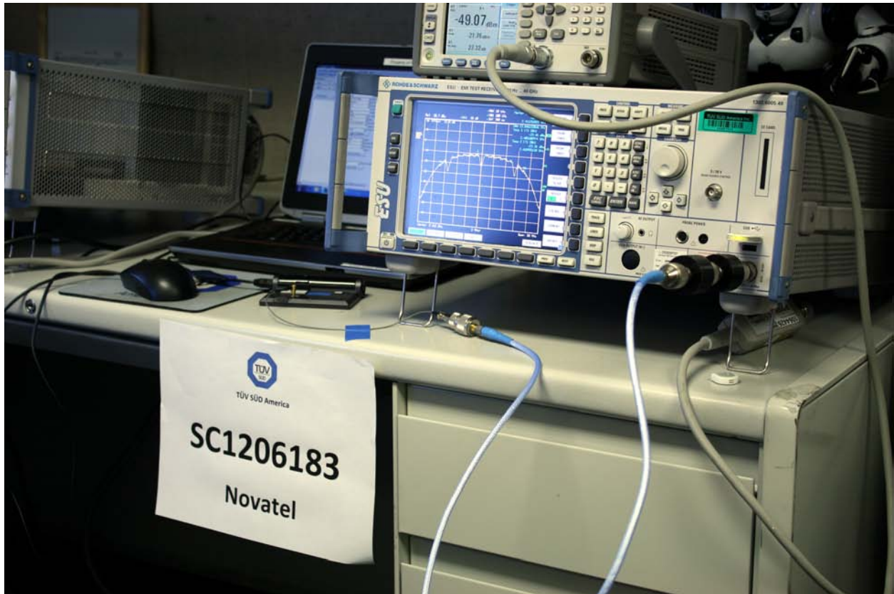
Conducted Port Measurement using spectrum analyzer (WiFi)
