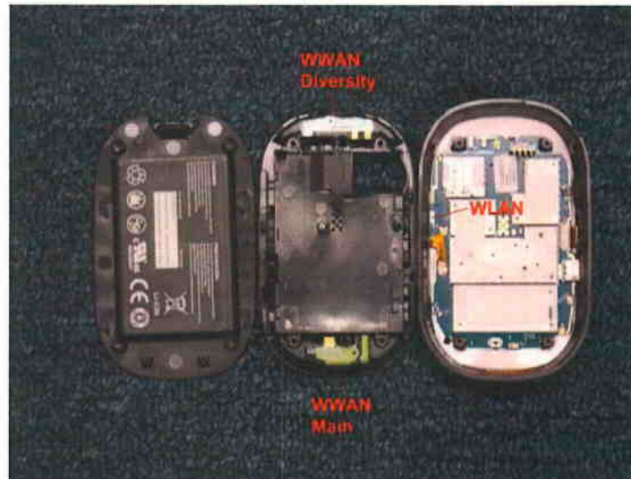
Antenna Location
