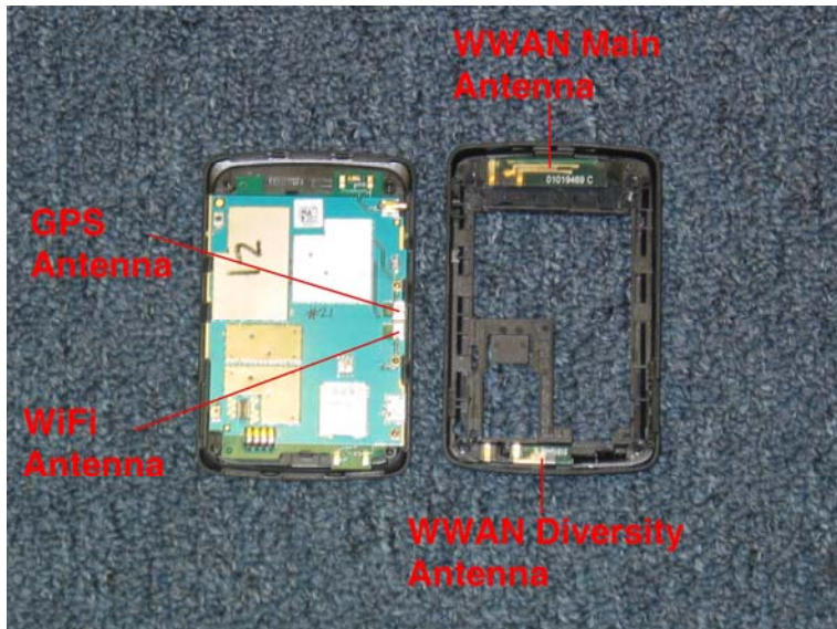
Antenna Locations
