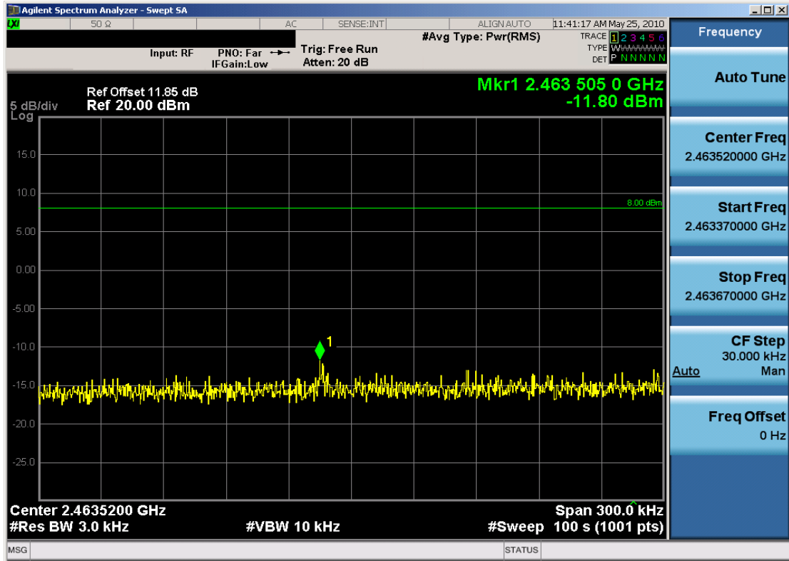
Plot 6-6. Power Spectral Density Plot (802.11b – Ch. 11)
