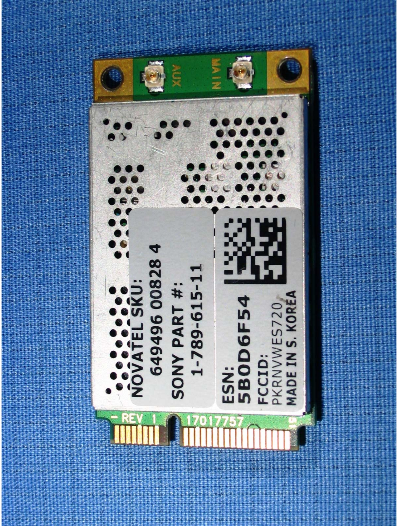
Figure 6: MCD3000 – Top of ES720 Radio
